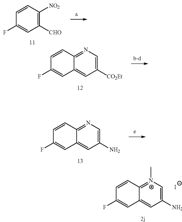
Scheme 3. Synthesis of certain C6-fluorinated quinolinium derivatives of the invention a
