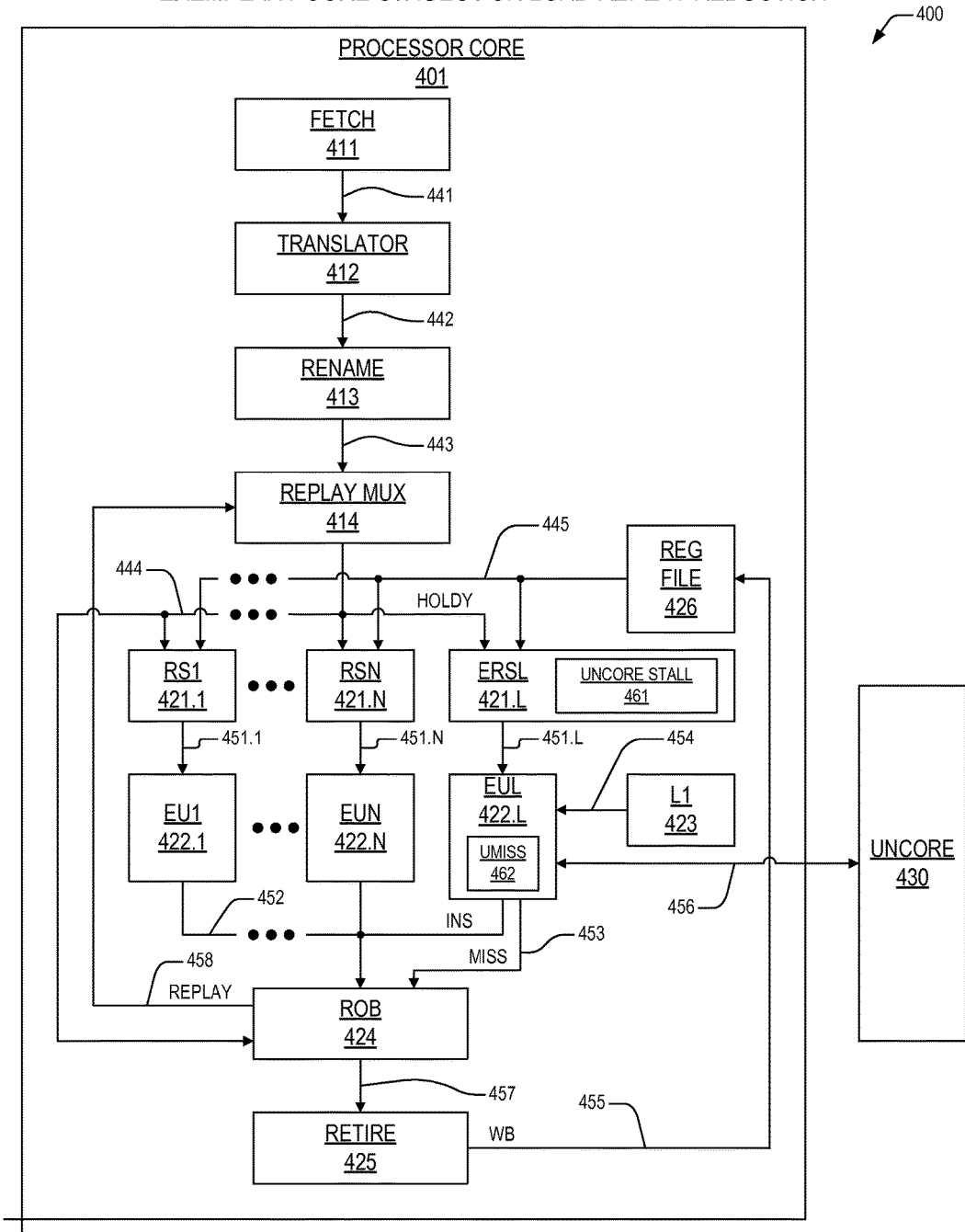
EXEMPLARY CORE STAGES FOR LOAD REPLAY REDUCTION
