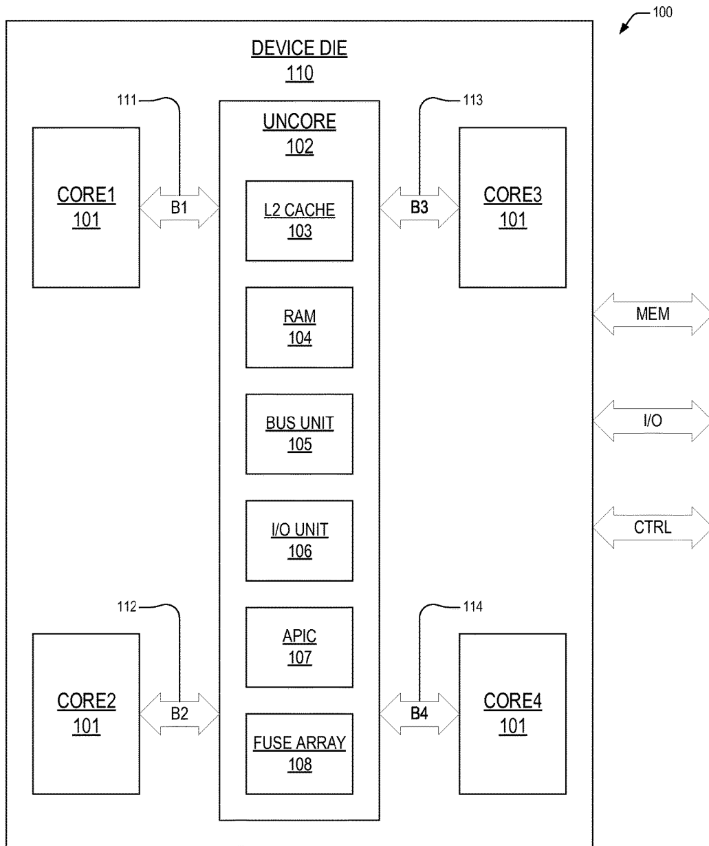
MULTI-CORE PROCESSOR WITH NON-CORE COMMON RESOURCES
