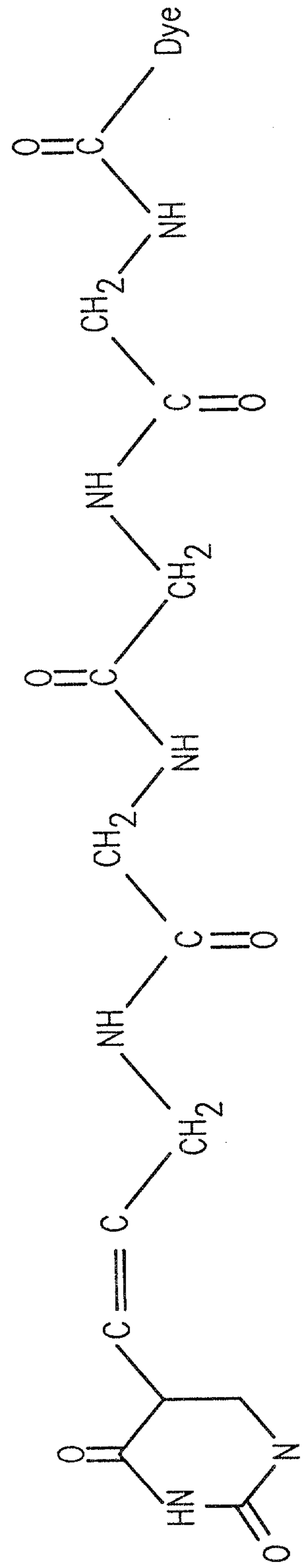
Tetraglycinylnyl linker
