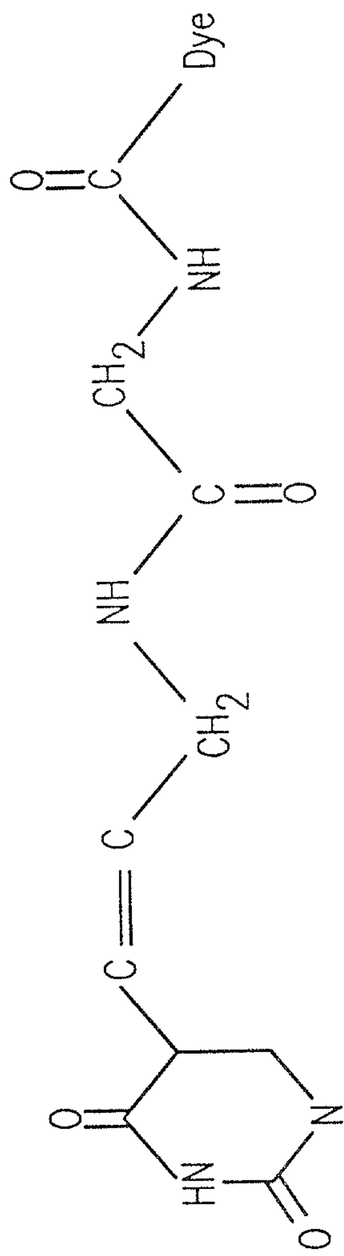
Diglycinylnyl linker
