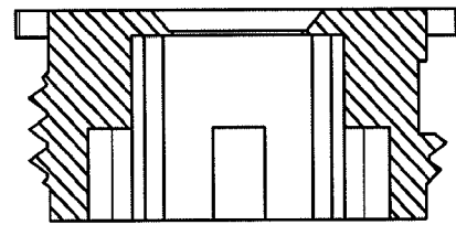
SECTION E-E
