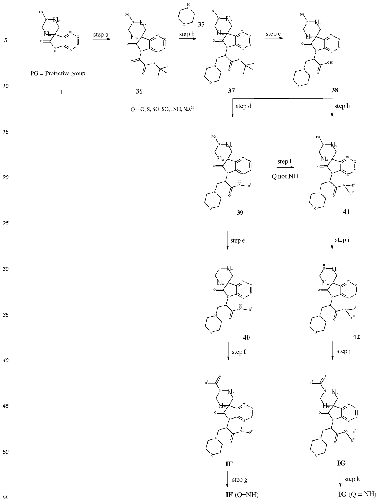
Scheme 9
