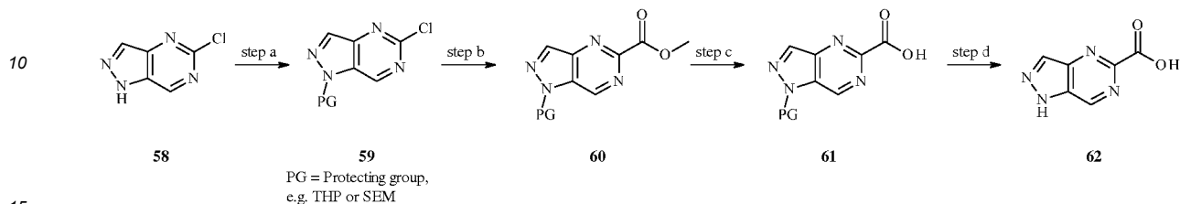
Scheme 12
