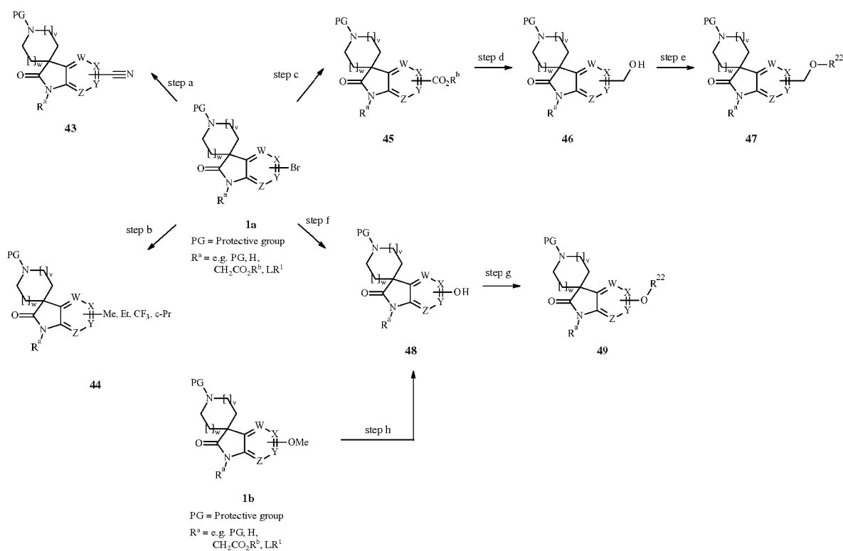
Scheme 10
