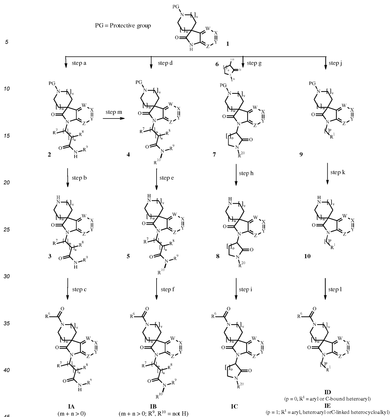
Scheme 1
