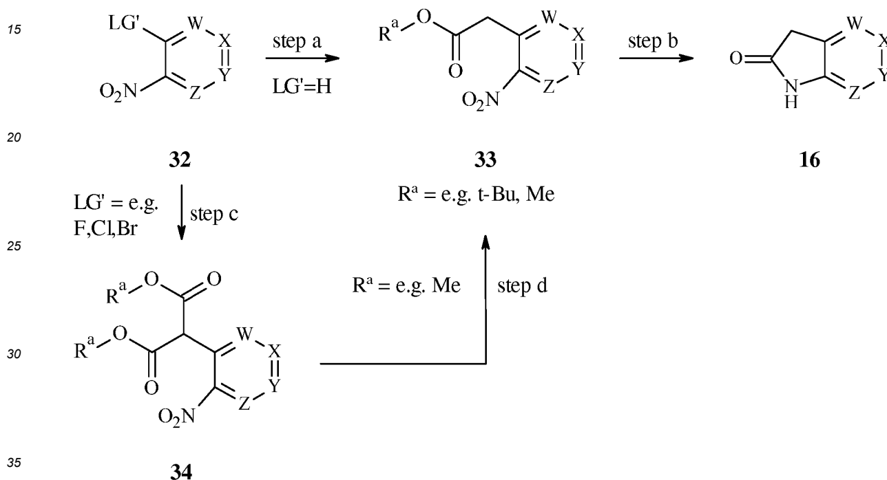
Scheme 8
