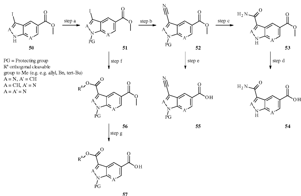
Scheme 11
