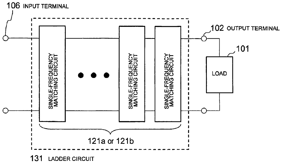
PRIOR ART FIG. 13
