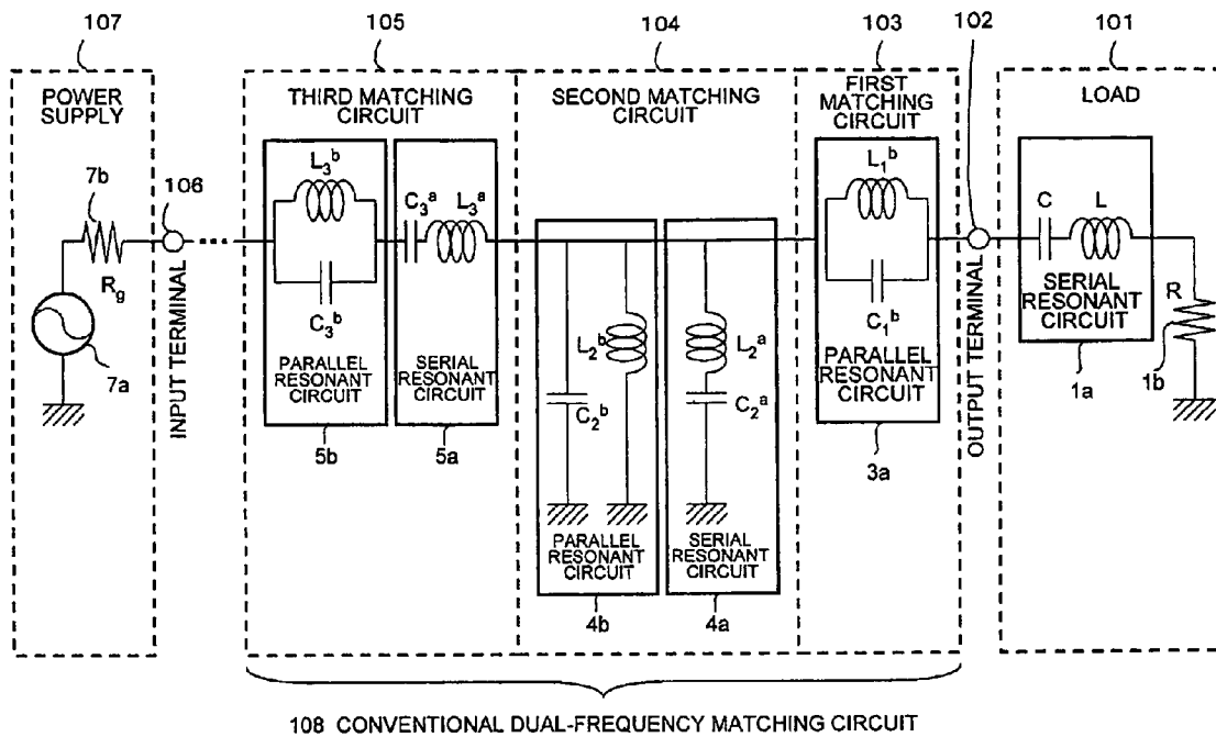
PRIOR ART FIG. 11
