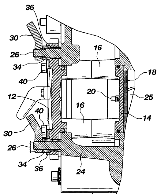
FIG. 2 (PRIOR ART)
