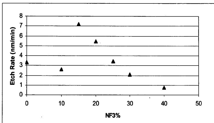
Figure 7b: \text{HfSi}_x\text{O}_y etch rates at different \text{NF}_3 by volume percentages in the gaseous mixture of \text{BCl}_3 and \text{NF}_3 .
