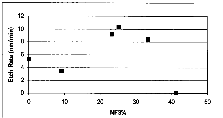
Figure 7a: \text{HfO}_2 etch rates at different \text{NF}_3 by volume percentages in the gaseous mixture of \text{BCl}_3 and \text{NF}_3 .
