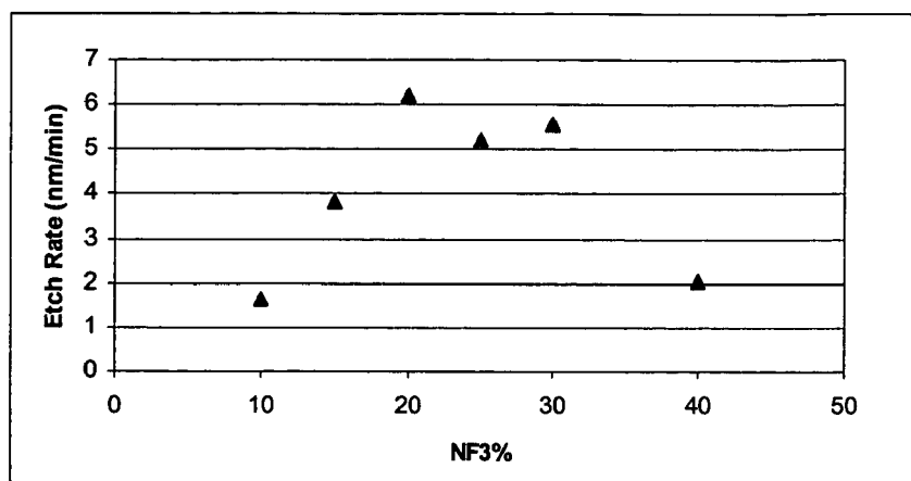
Figure 7c: ZrO 2 etch rates at different NF 3 by volume percentages in the gaseous mixture of BCl 3 and NF 3 .
