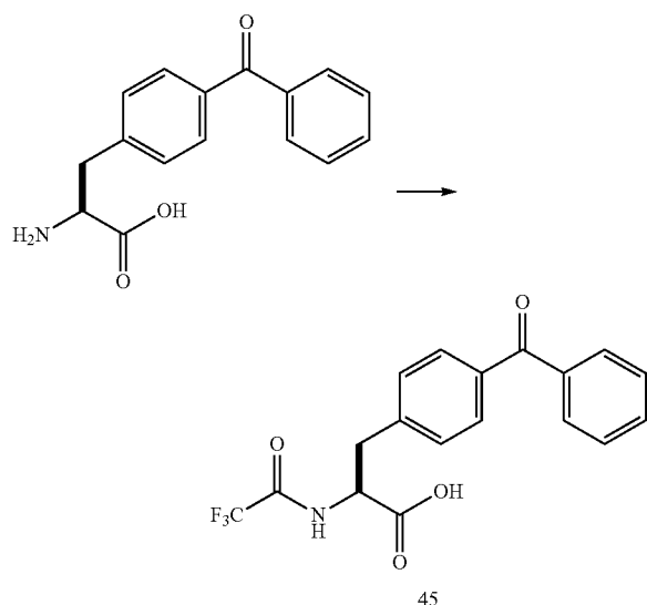
N-Trifluoroacetyl 4-benzoylphenylalanine (45)
