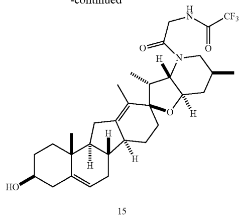
N-(N'-Trifluoroacetyl glycyl)cyclopamine (15)
