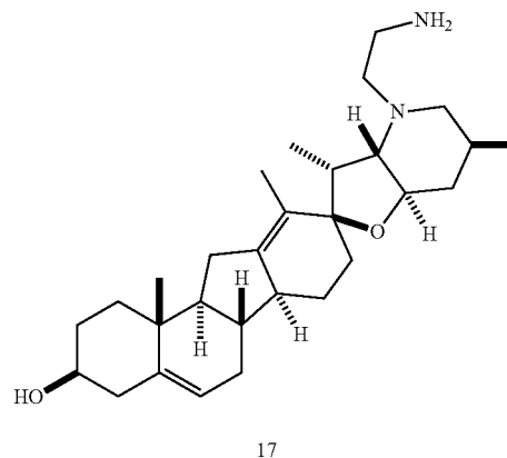
N-Aminoethyl cyclopamine (17)
