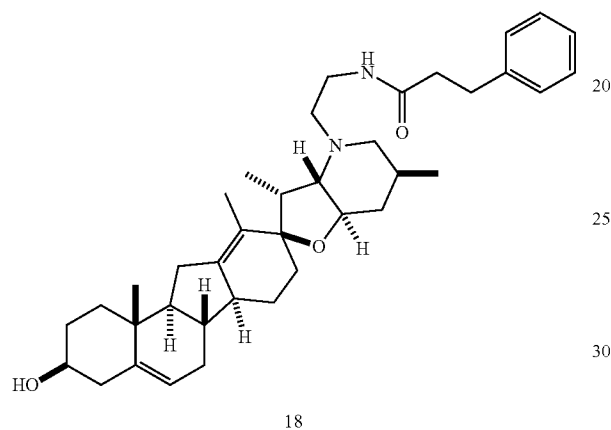
N—(N'-Dihydrocinnamoyl aminoethyl)cyclopamine (18)
