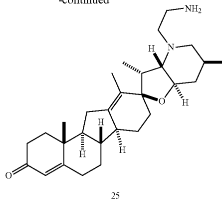
3-Enone, N-aminoethyl cyclopamine (25)
