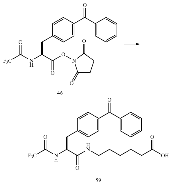
N—(N'-Trifluoroacetyl(4-benzoylphenylalanine)) aminocaproic acid (59)
