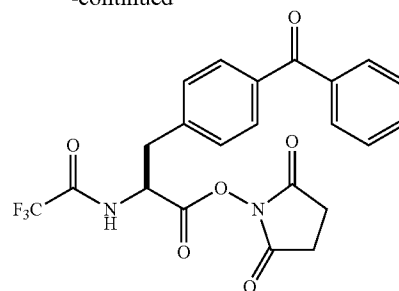
N-Trifluoroacetyl 4-benzoylphenylalanine N-hydroxysuccinimide ester (46)
