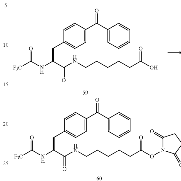
N—(N'-Trifluoroacetyl(4-benzoylphenylalanine)) aminocaproic acid N-hydroxysuccinimide ester (60)
