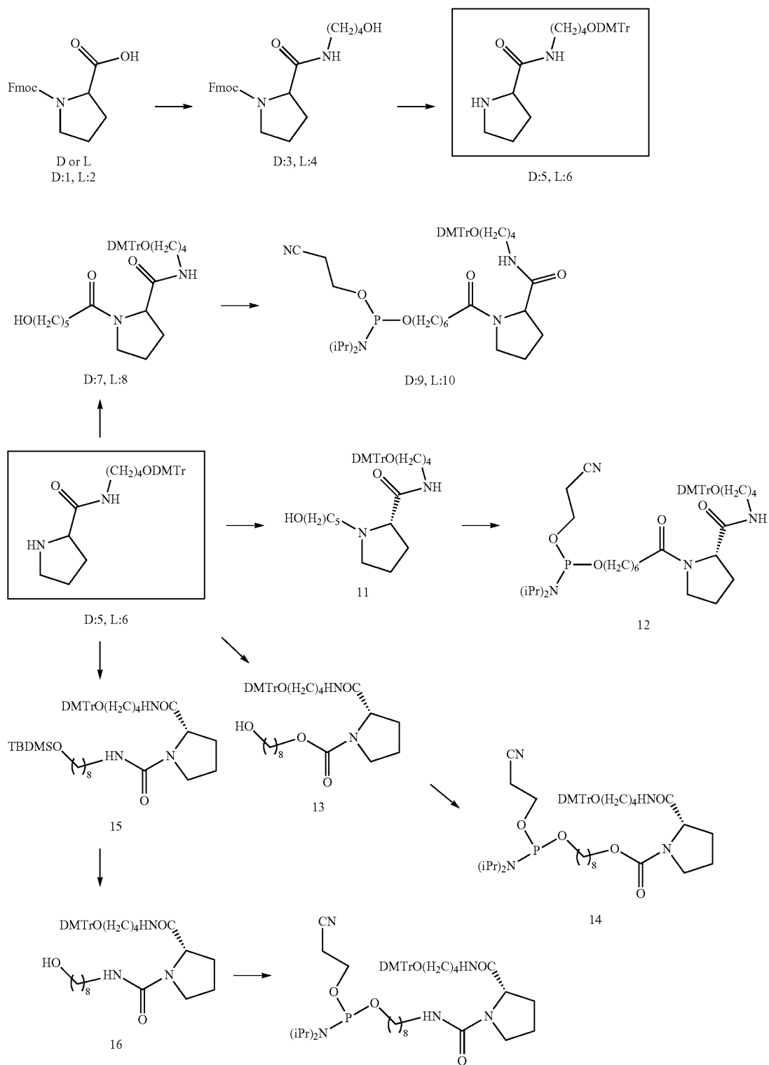
Scheme 3
