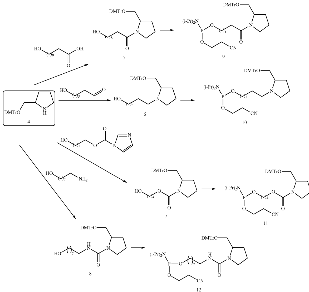
Scheme 2
