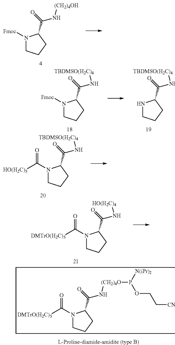
Scheme 4
