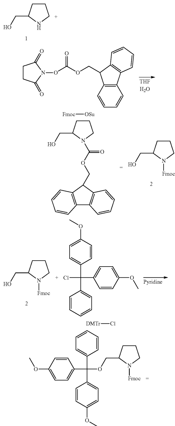
Scheme 1
