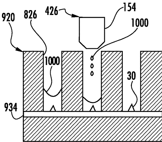
DISPENSE ANALYTE AND INCUBATE FIG. 11
