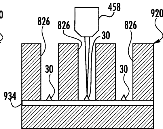
OBTAIN SERS SPECTRA FIG. 16
