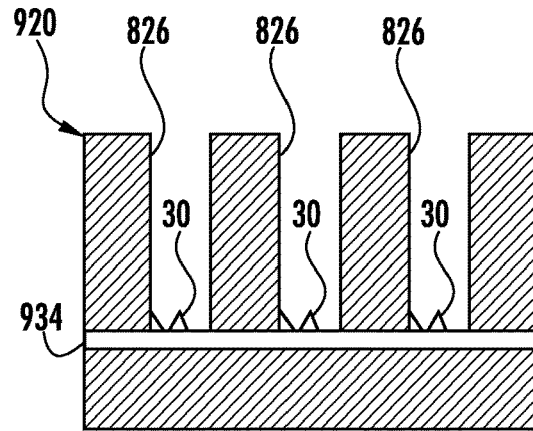
VACUUM ANALYTE SOLUTION FIG. 12
