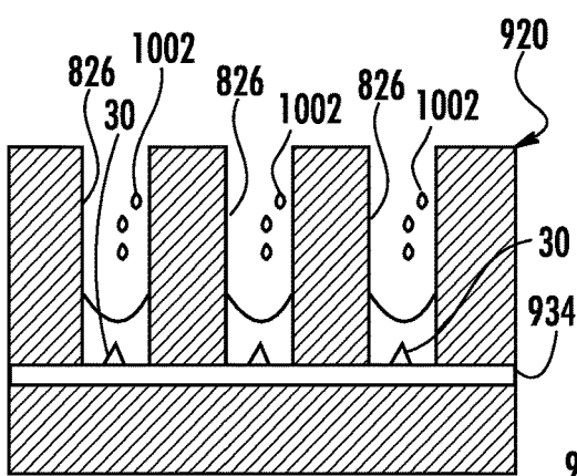
DISPENSE RINSING SOLVENT AND CLOSE NANOFINGERS FIG. 13
