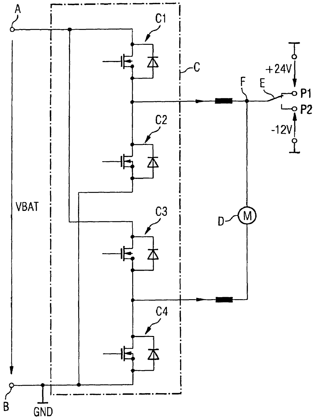
FIG 5 Prior Art
