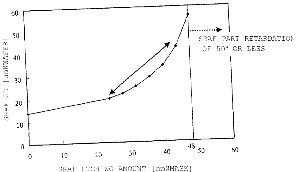
RELATION BETWEEN ETCHING AMOUNT AND SRAF DIMENSION
