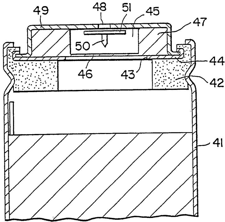
FIG. 2 PRIOR ART
