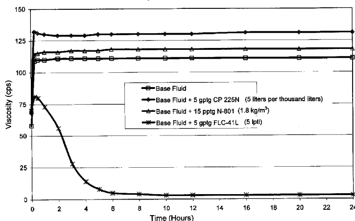
FIG. 1 - Viscosity Tests for VES fluids at 160°F (66°C) and 100 1/s Base Fluid: Tap water + 4%bv WG-3L + 3%bw KCl
