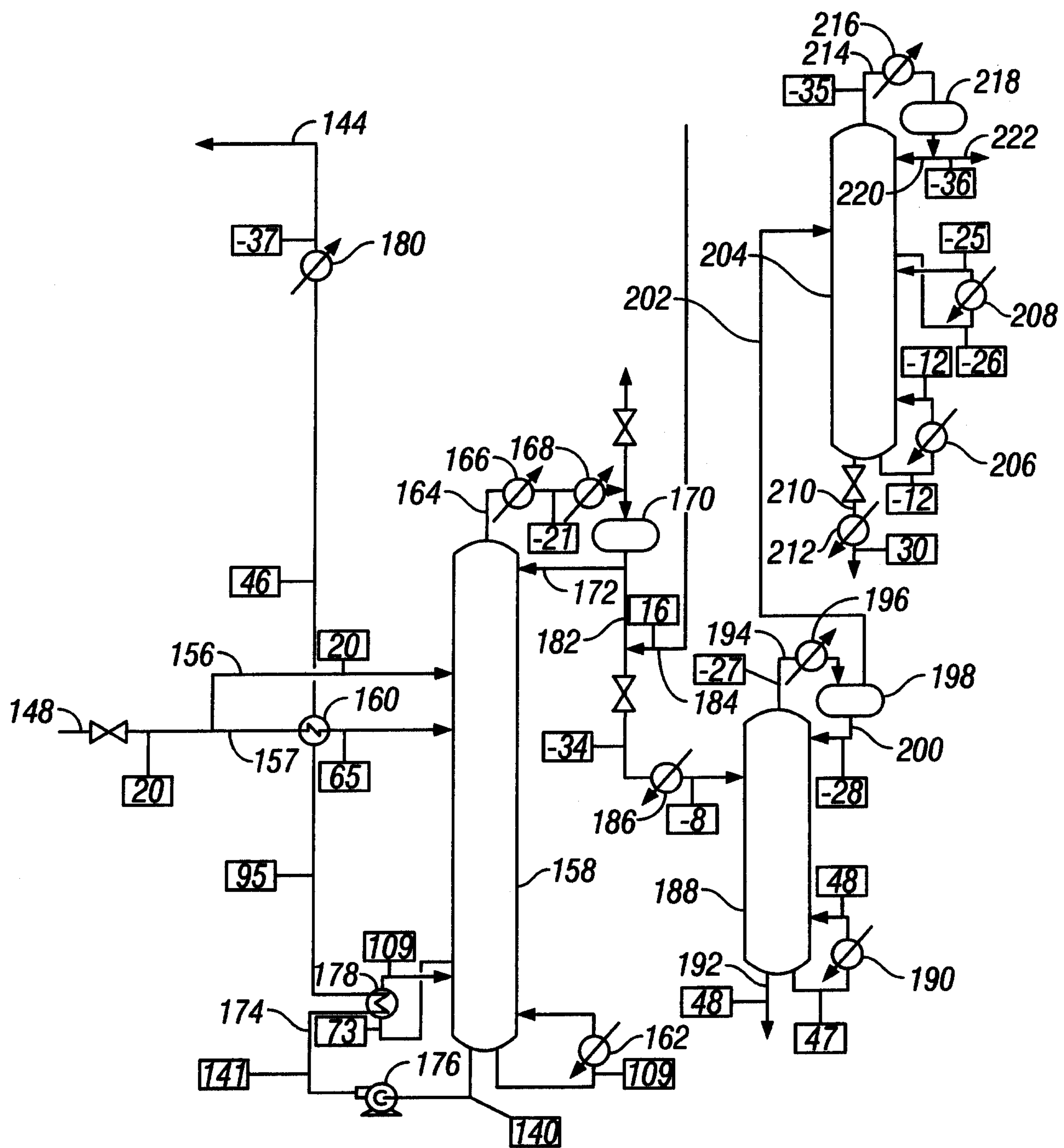
FIG. 2 (Prior Art)
