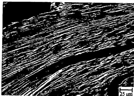
Anisotropic - Needle Coke
