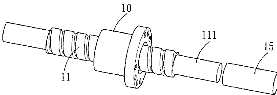
FIG. 5 PRIOR ART
