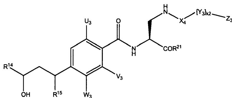
Formula V
