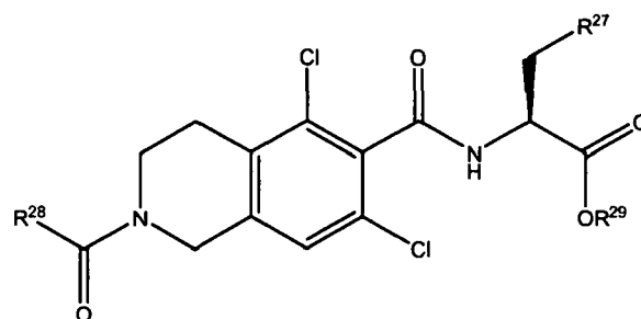
Formula II'
