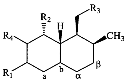
Formula X
