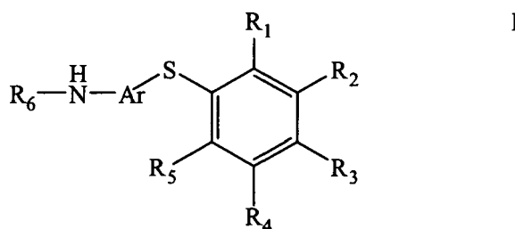
Formula VII
