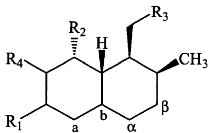
Formula XI
