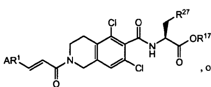
Formula IIA
