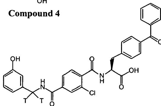
Compound 5
