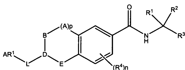
Formula 1
