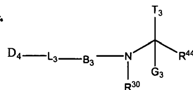
Formula VI
