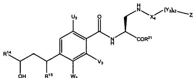
Formula V
