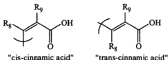
Formula VII-c
