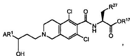
Formula IA
