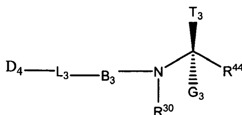
Formula VI
