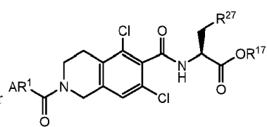
Formula IIB
