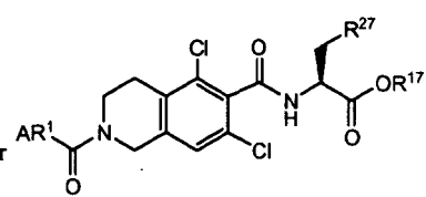
Formula IIB
