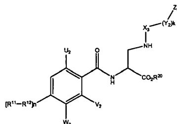
Formula IV
