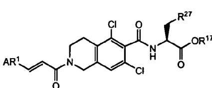
Formula IIA
