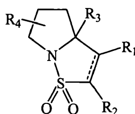
Formula IX
