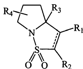
Formula IX
