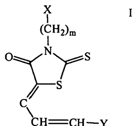
Formula VIII
