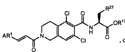
Formula IIA
