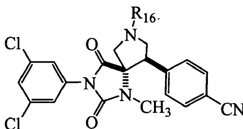
Formula XI
