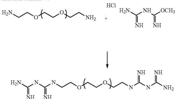
Reaction Scheme V:
