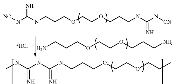
Reaction Scheme I:
