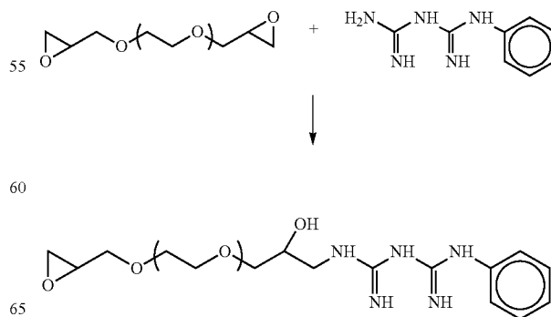
Reaction Scheme IV:
