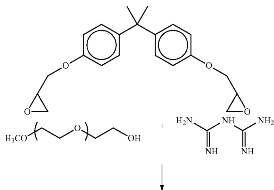
Reaction Scheme VI:
