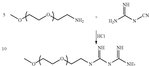
Reaction Scheme III:
