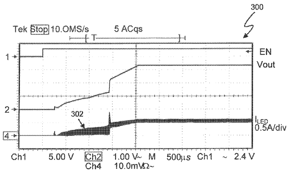
Figure 3 (Prior Art)
