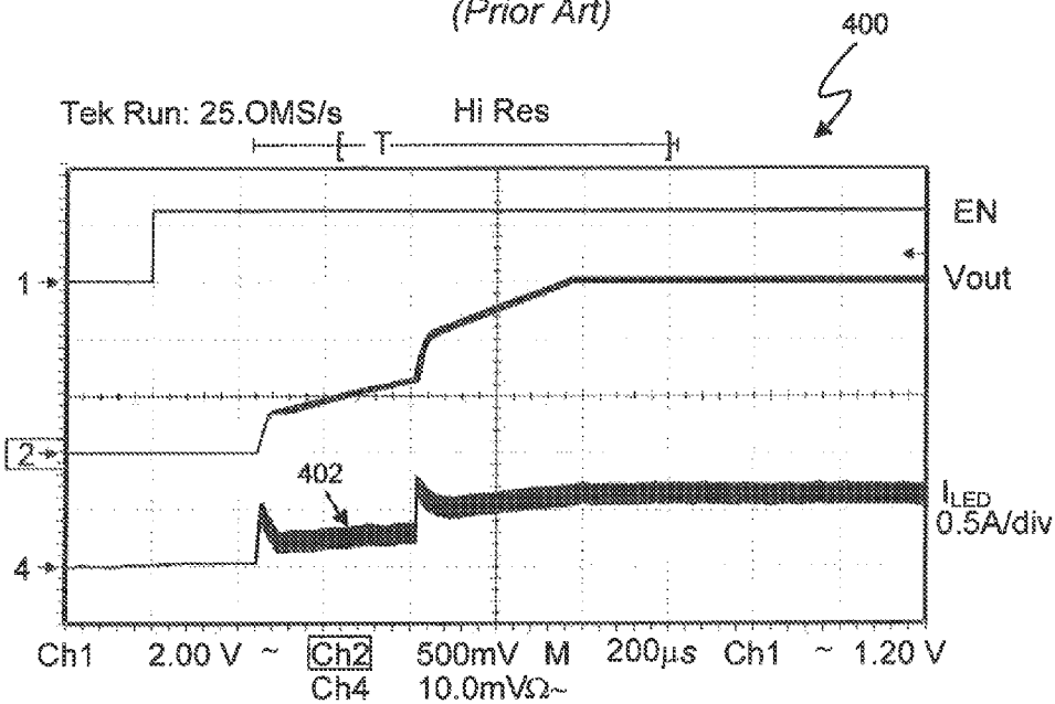
Figure 4 (Prior Art)
