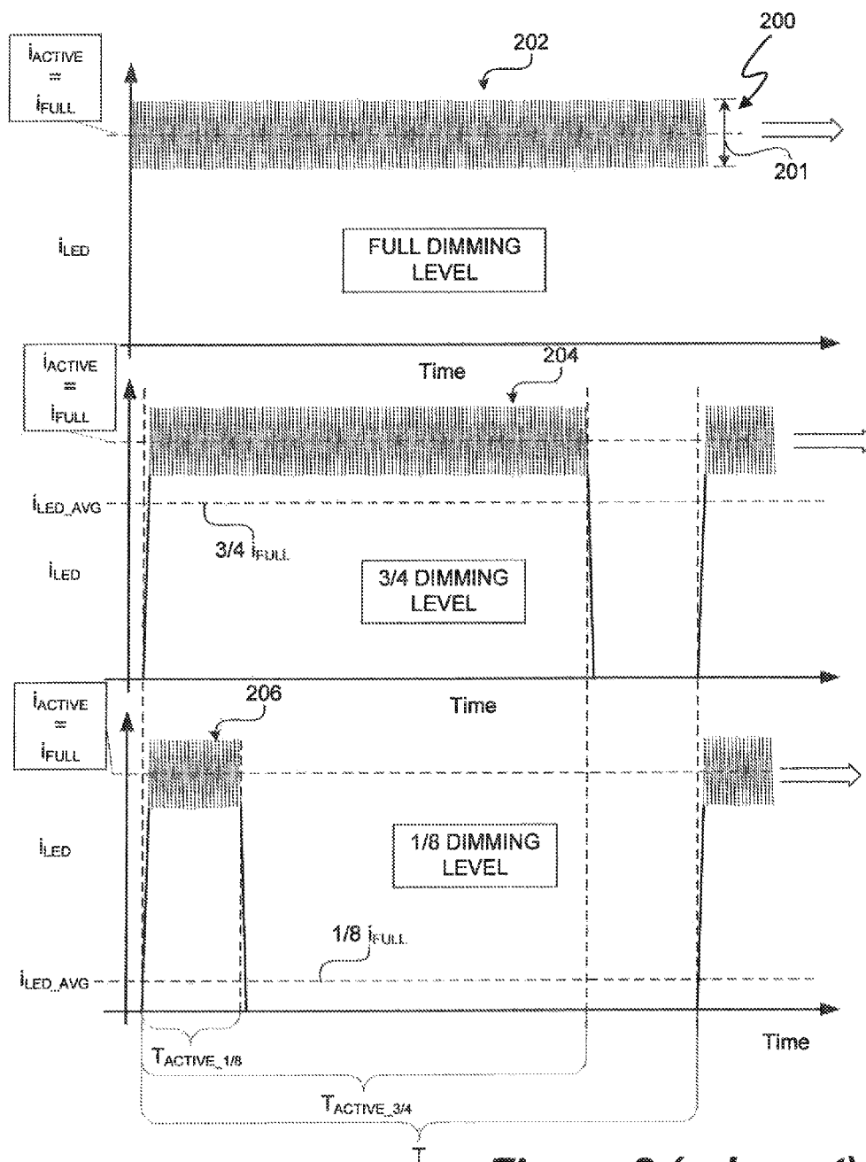
Figure 2 (prior art)
