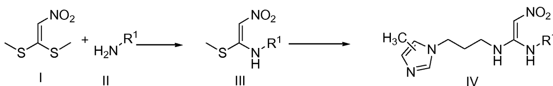
Scheme 1: General synthesis
