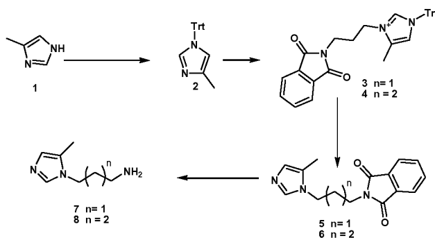
5 Scheme 1: Synthesis of 3-(5-methyl-1H-imidazol-1-yl)propan-1-amine (7)
