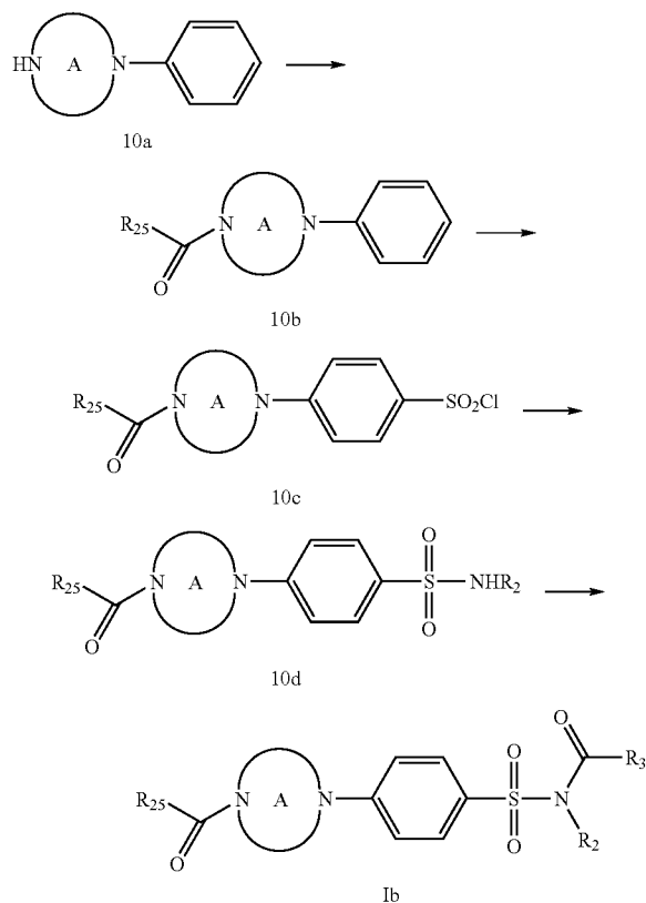
Scheme 10:
