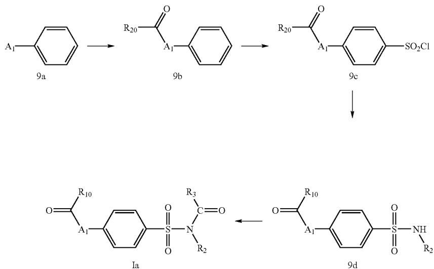
Scheme 9:
