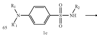
Scheme 13:
