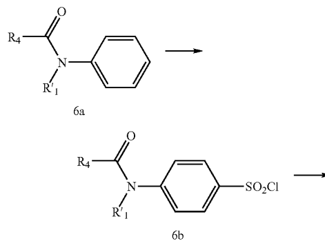
Scheme 6:
