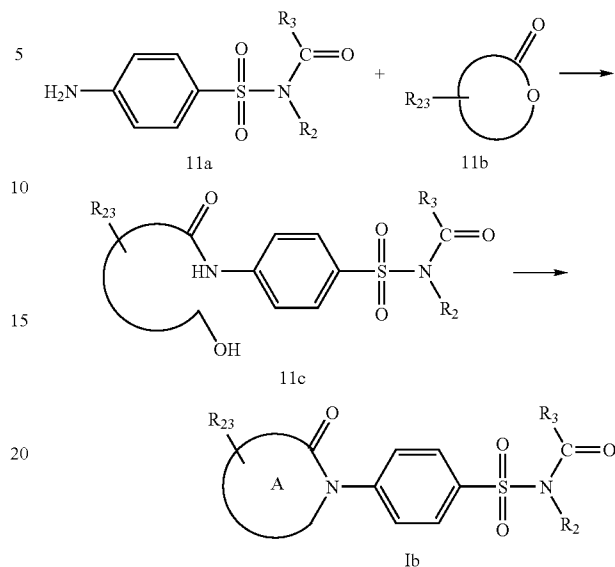
Scheme 11:
