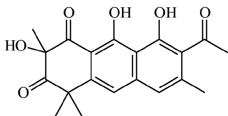
2-hydroxyGarveatin A
