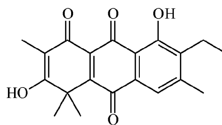
Garveatin B quinone
