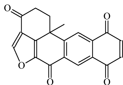
Helenaquinone
