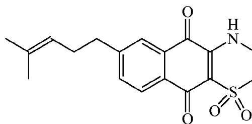
Conicaquinone B
