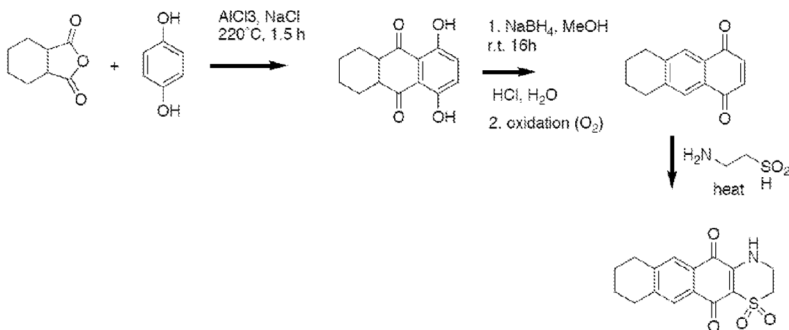
Scheme IV
