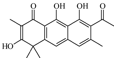
Garveatin A
