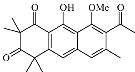
Garveatin C
