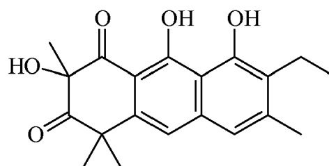
2-hydroxyGarveatin B
