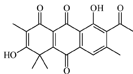
Garveatin A quinone
