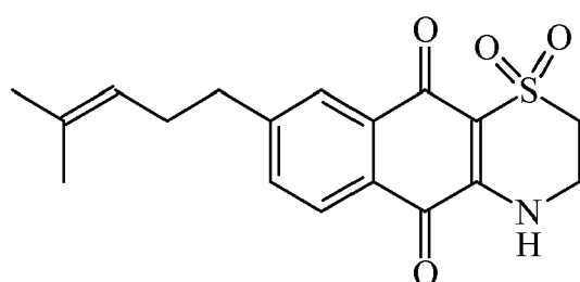
Conicaquinone A
