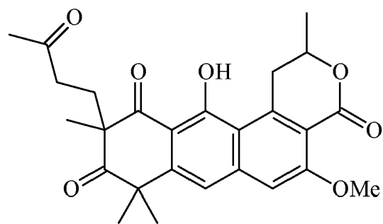
Garvalone B
