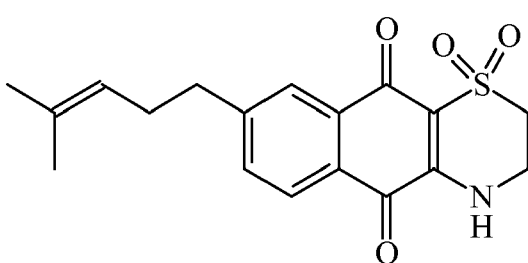
Conicaquinone A
