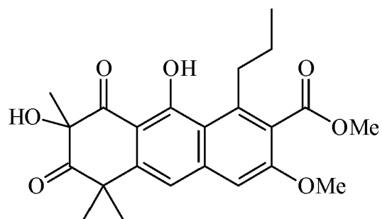
2-hydroxygarvin A
