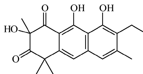
2-hydroxyGarveatin B
