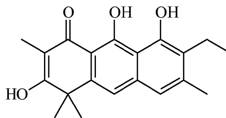
Garveatin B
