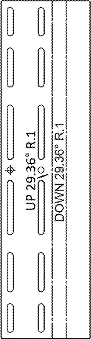
FLAT PATTERN
