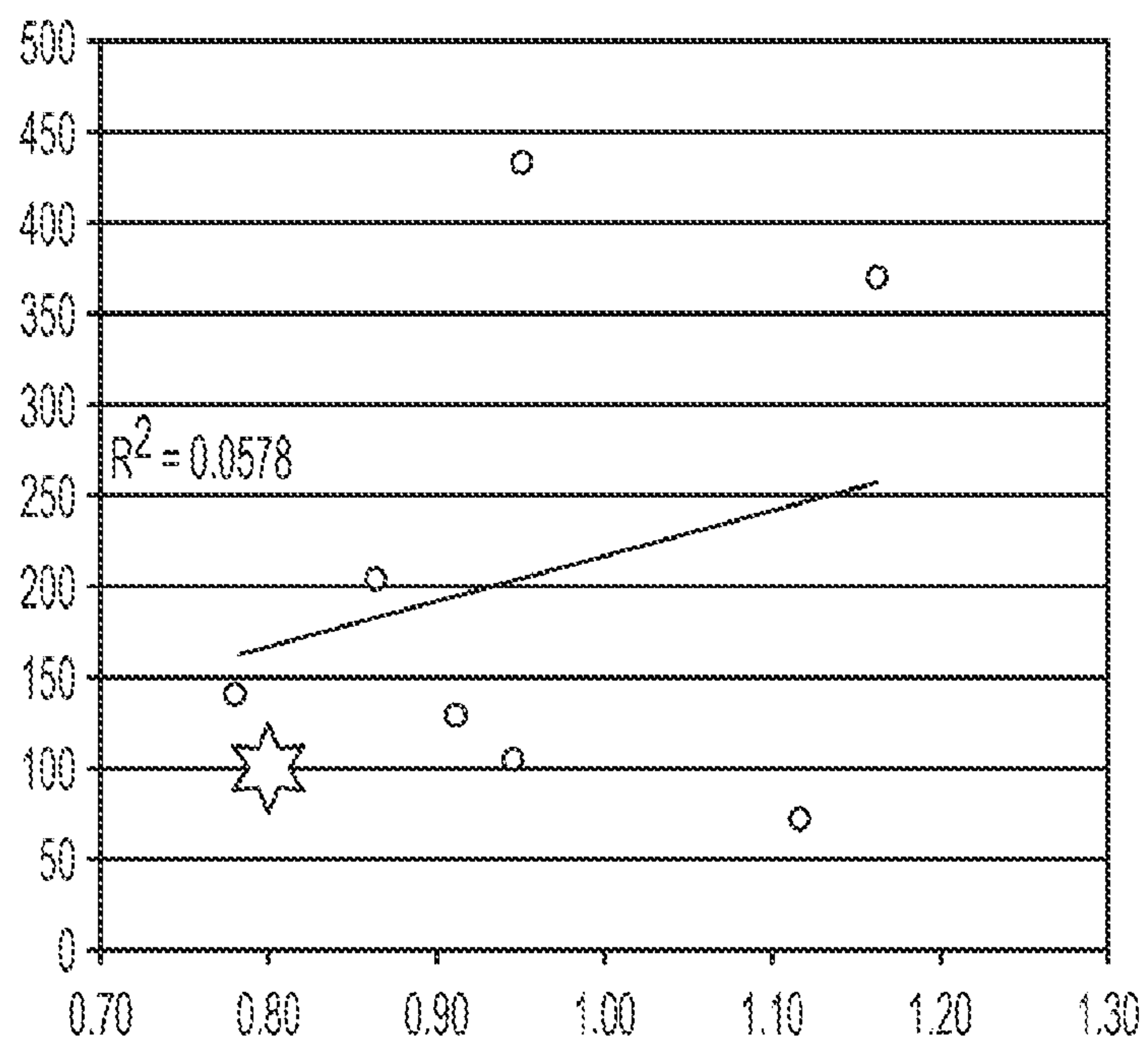
B/BRISBANE/60/2008 DRUG PRODUCT AUC OVER TRITON:HA RATIO
