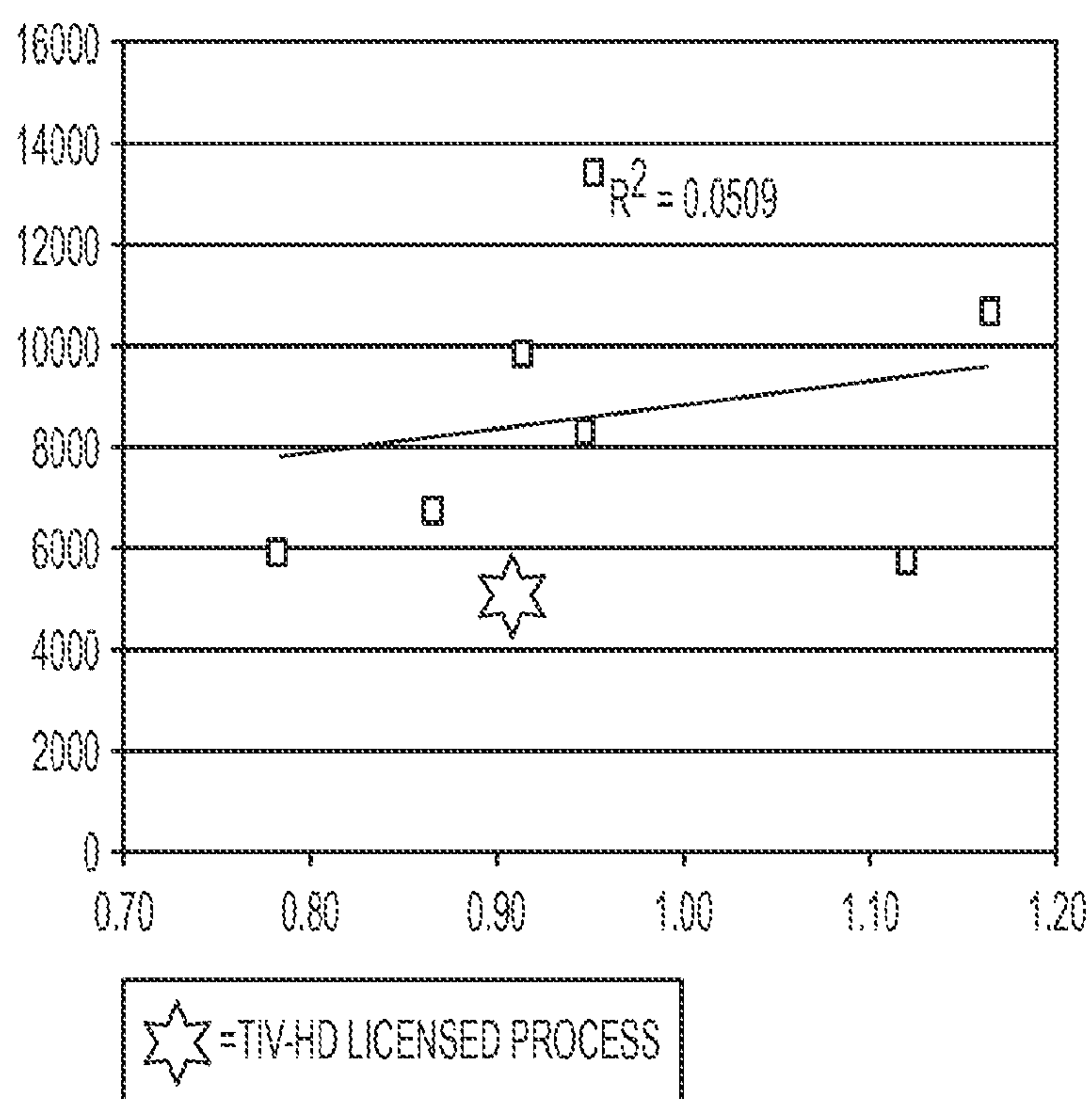
A/TEXAS/50/2012 DRUG PRODUCT AUC OVER TRITON:HA RATIO
