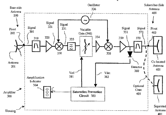
Circuit for Interference Repeater
