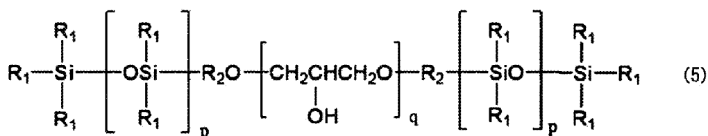
[Chemical Formula 4]
