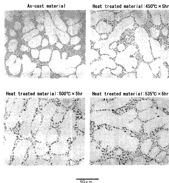
Figure 1 State of crystallized products in AC4CH as-cast material and heat-treated material
