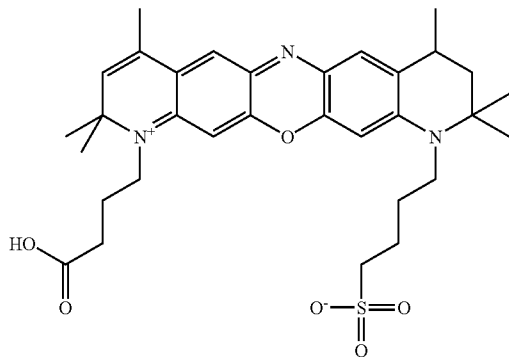
Structure of the JA286 dye
