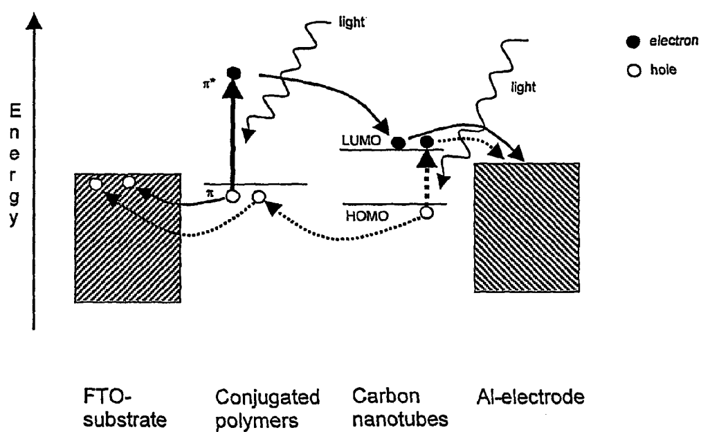
Fig. 2: Schematic band diagram and different excitation processes of and in a carbon nanotube based photovoltaic device according to the present invention.
