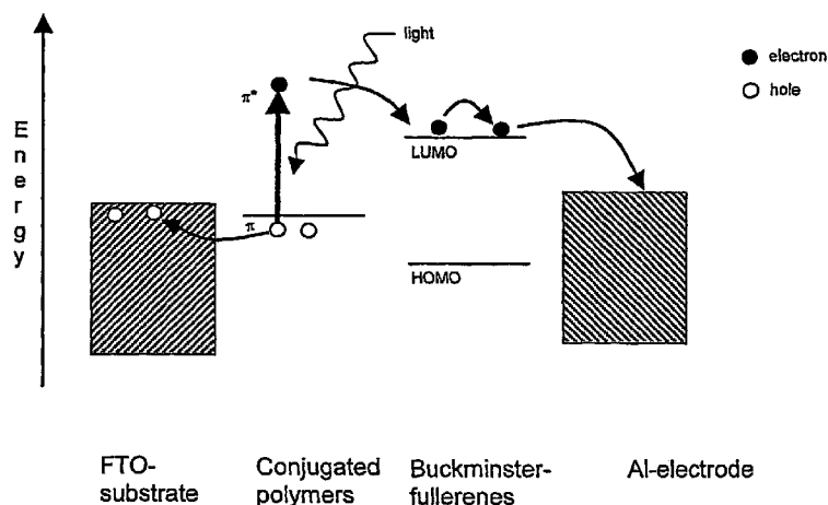
Schematic band diagram and different excitation processes of and in solar cells based on Buckminsterfullerenes.
