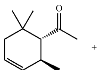
1-(2,6,6-trimethyl-3-cyclohexen-1-yl)-2-ethanone Mw = 166
