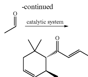
1-(2,6,6-trimethyl-3-cyclohexen-1-yl)-2-buten-1-one Mw = 192
