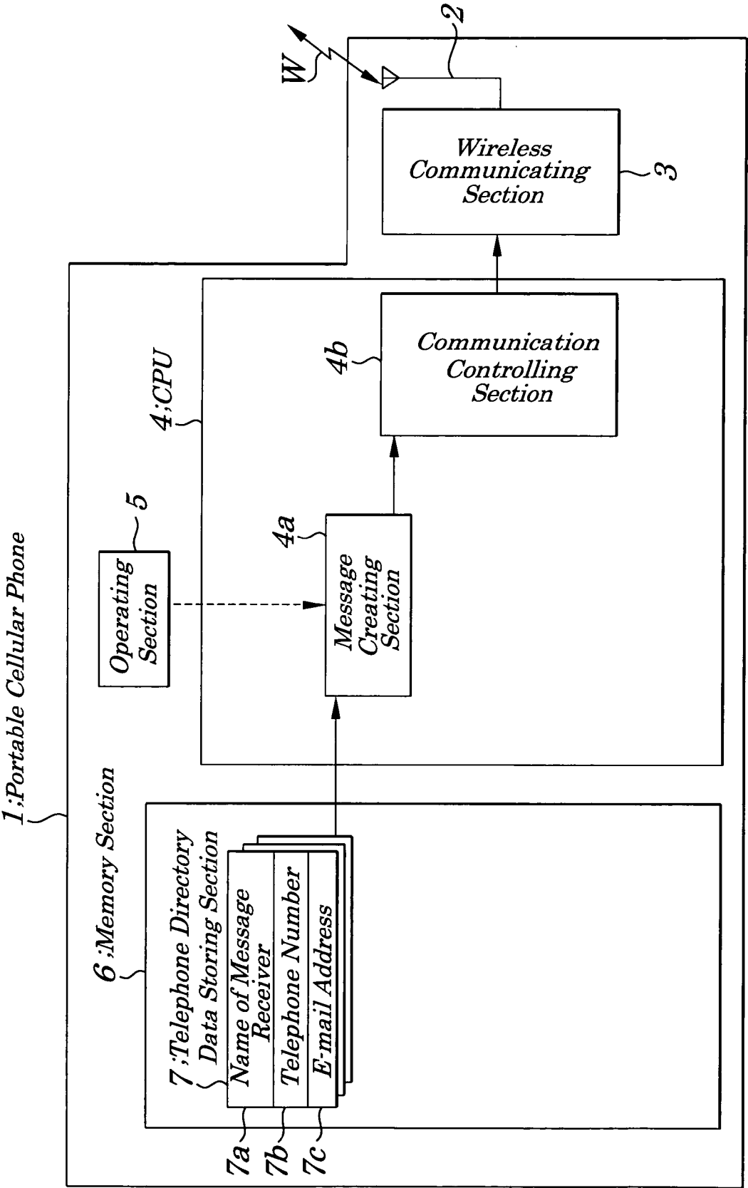
FIG.3 (PRIOR ART)
