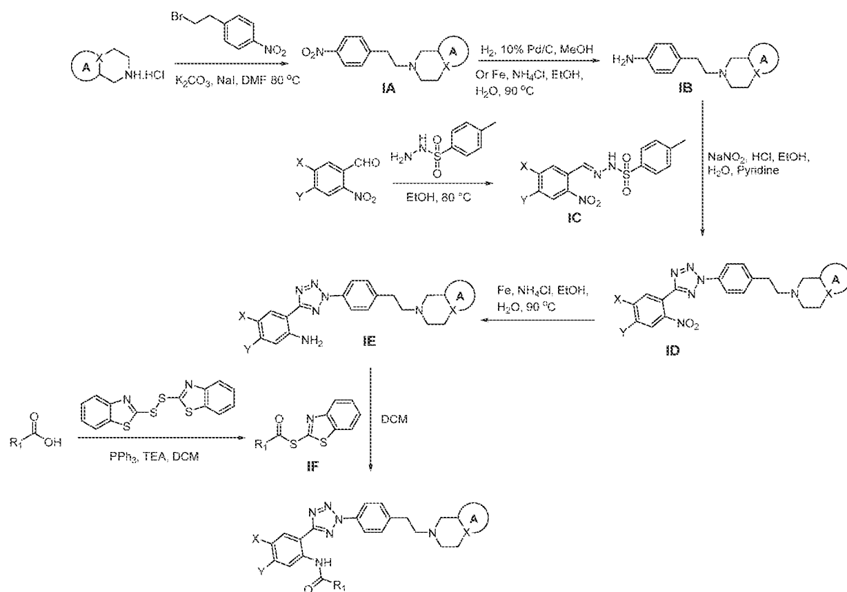
Scheme 1
