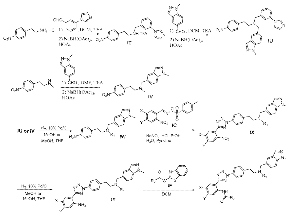
Scheme 4
