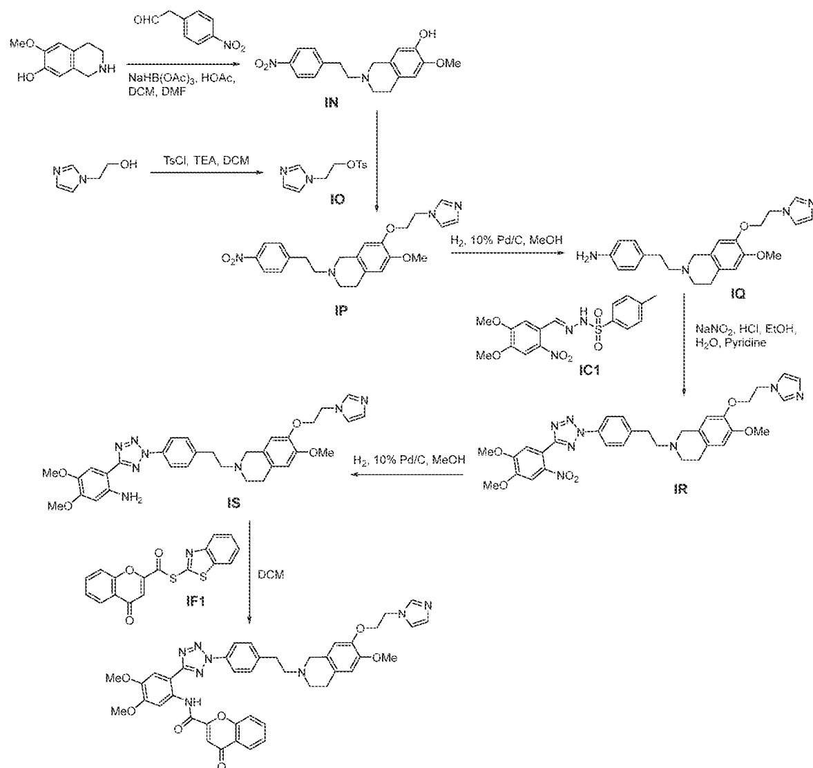
Scheme 3
