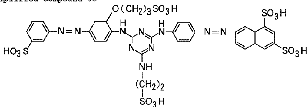
Exemplified Compound 35
