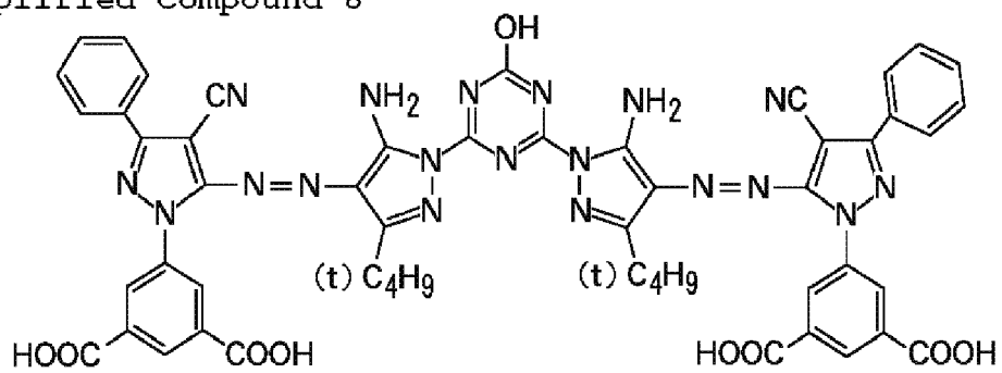
Exemplified Compound 8
