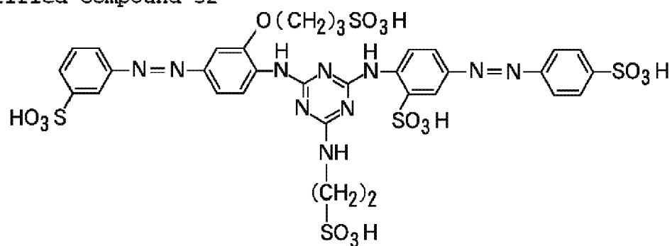
Exemplified Compound 32
