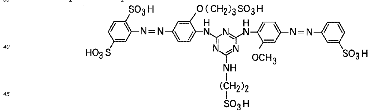
Exemplified Compound 23
