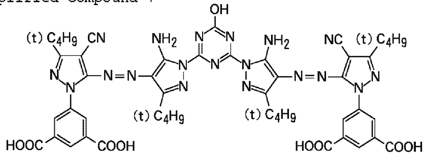
Exemplified Compound 7
