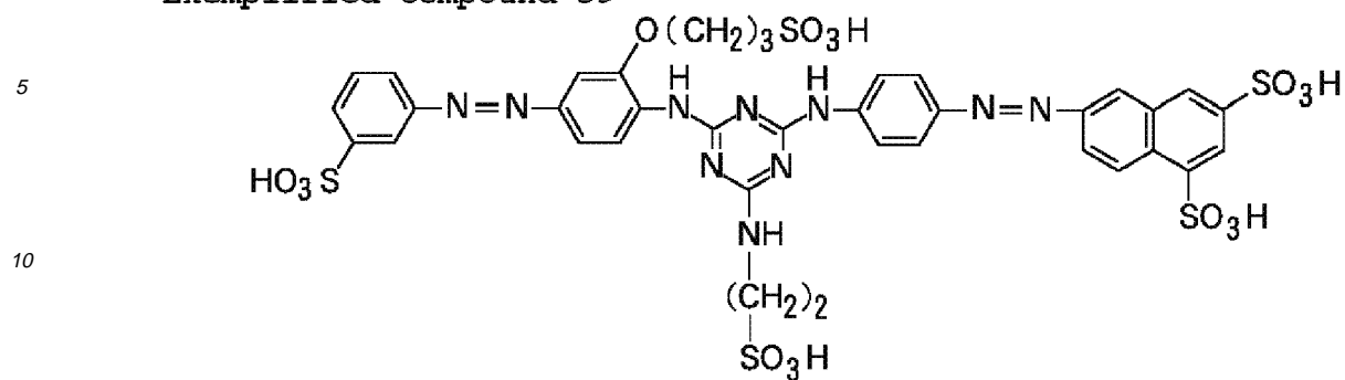
Exemplified Compound 39
