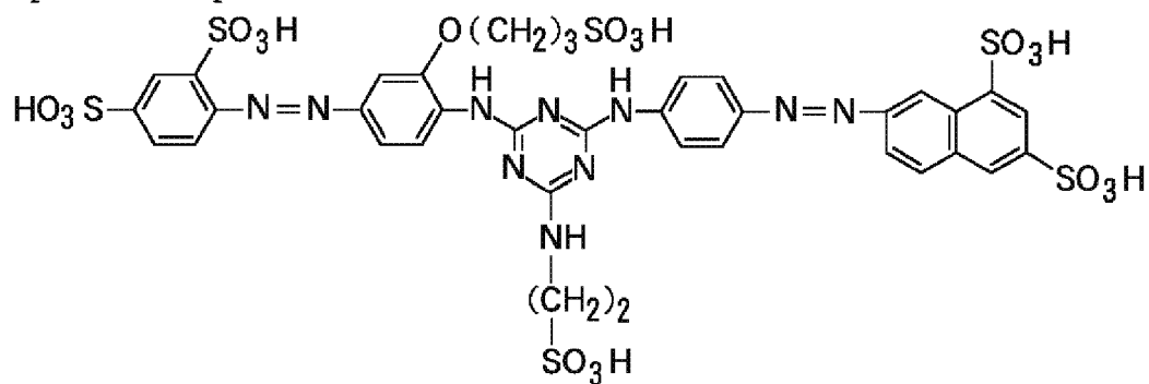
Exemplified Compound 37
