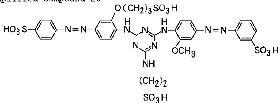
Exemplified Compound 20
