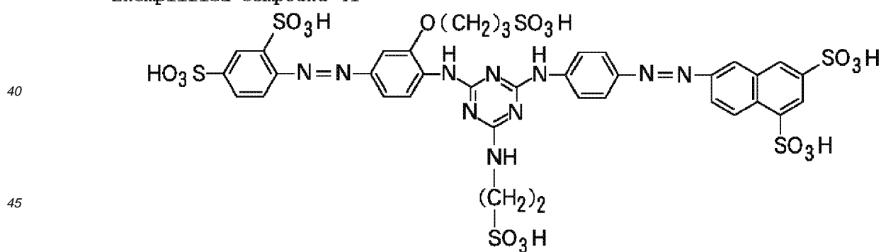
Exemplified Compound 41
