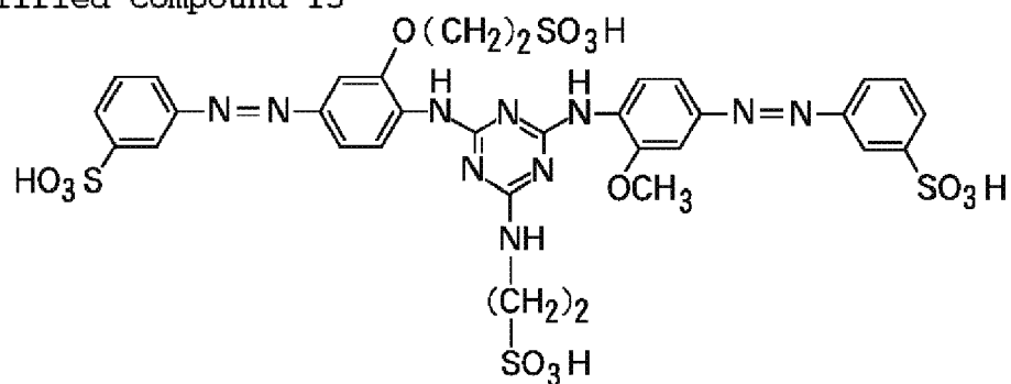
Exemplified Compound 15
