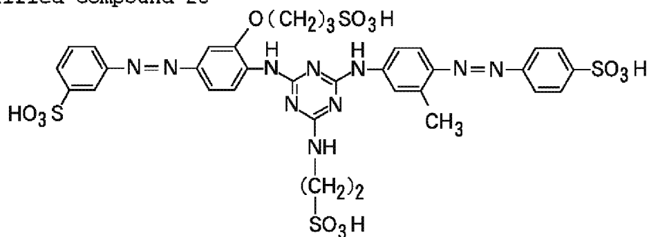
Exemplified Compound 28
