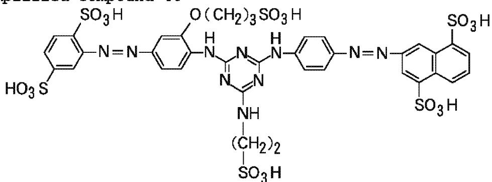
Exemplified Compound 46
