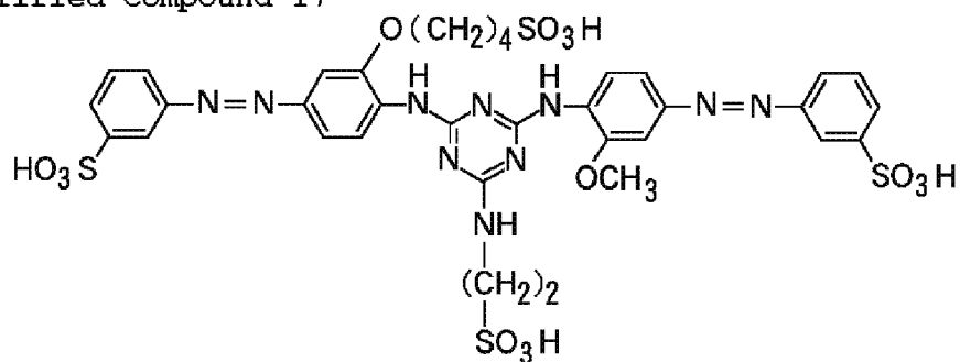
Exemplified Compound 17
