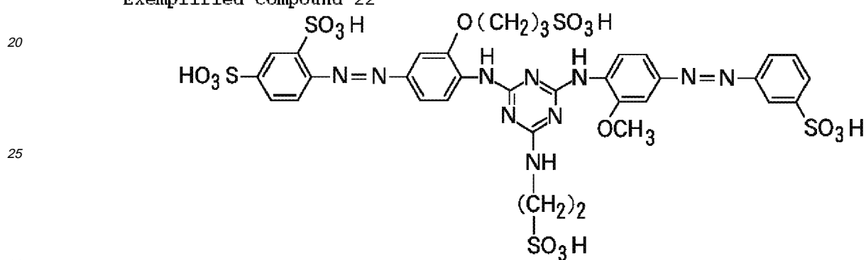
Exemplified Compound 22
