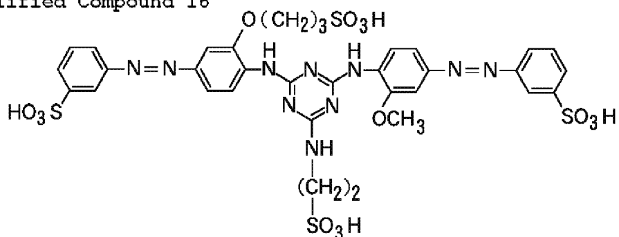
Exemplified Compound 16
