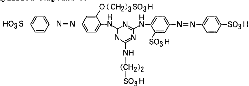
Exemplified Compound 33
