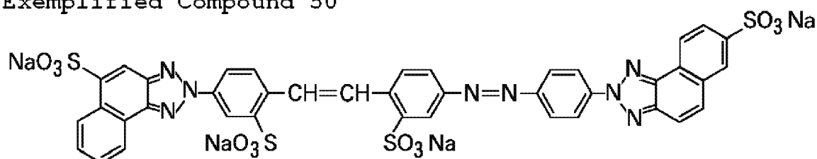
Exemplified Compound 50
