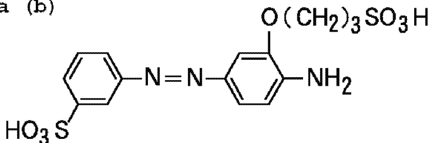
Formula (b)
