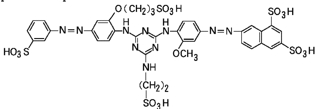
Exemplified Compound 47
