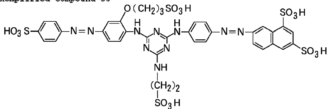
Exemplified Compound 36
