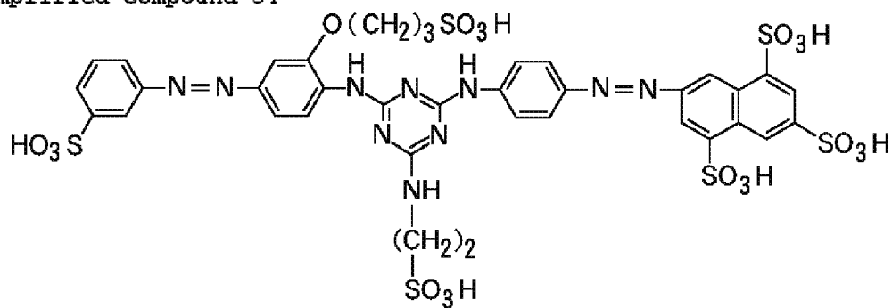
Exemplified Compound 34
