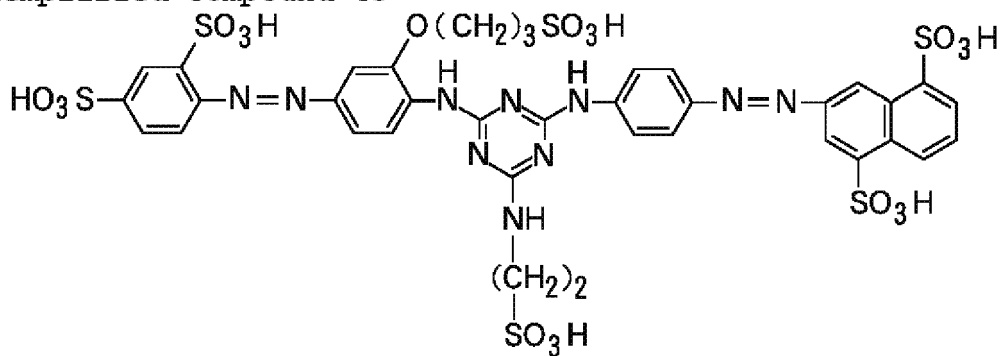
Exemplified Compound 45
