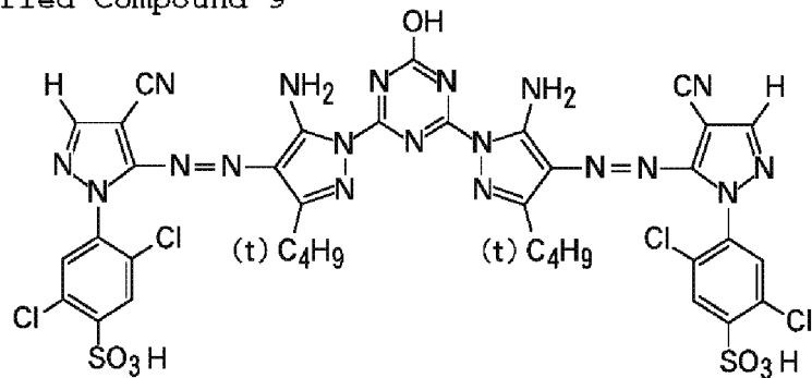
Exemplified Compound 9
