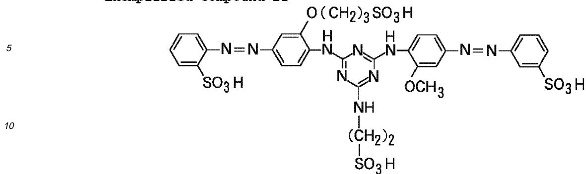
Exemplified Compound 21
