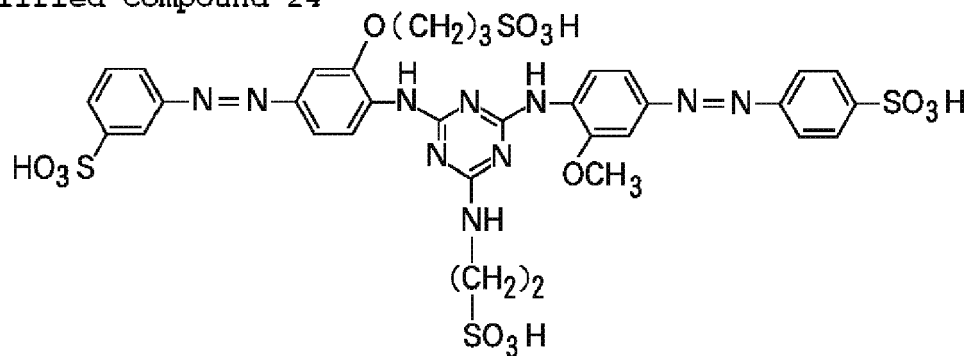
Exemplified Compound 24
