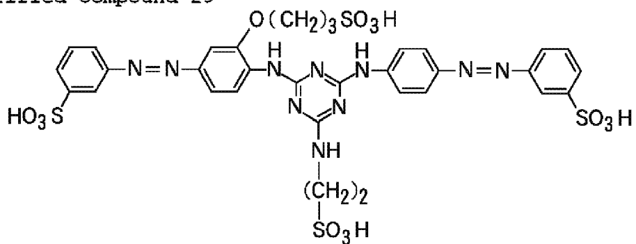
Exemplified Compound 29
