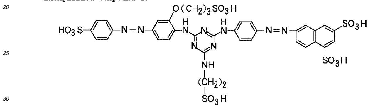
Exemplified Compound 40
