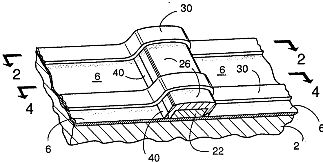
Figure 3 (PRIOR ART)
