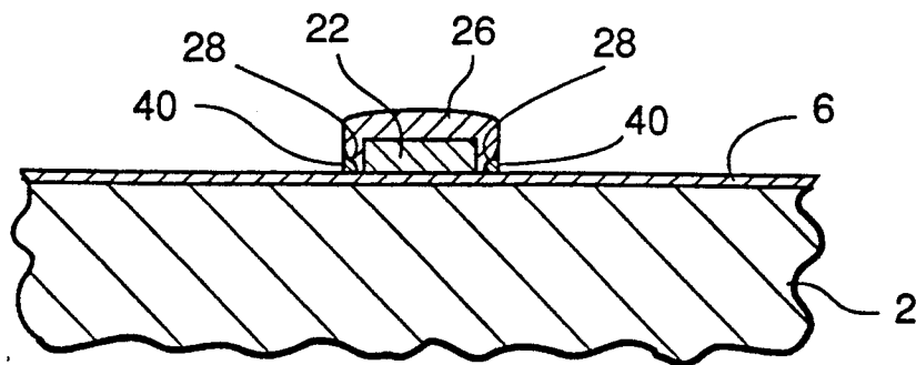
Figure 4 (PRIOR ART)
