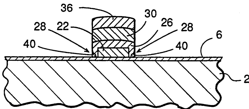
Figure 2 (PRIOR ART)
