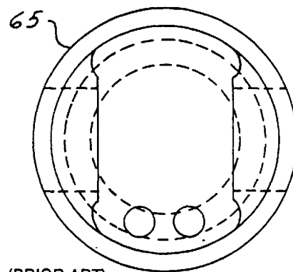
(PRIOR ART) FIG. 7C
