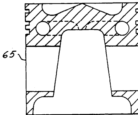
(PRIOR ART) FIG. 7A
