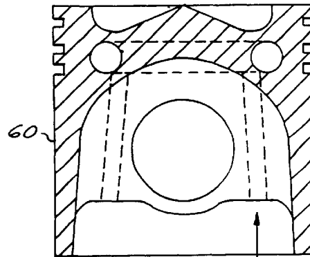
(PRIOR ART) FIG. 6B
