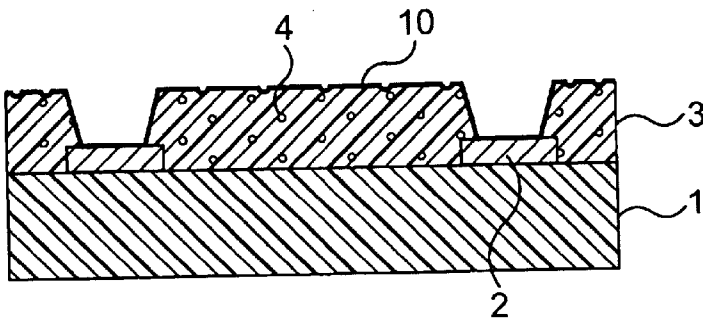
FIG. 4(f) PRIOR ART
