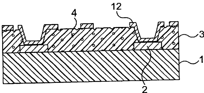
FIG. 4(h) PRIOR ART
