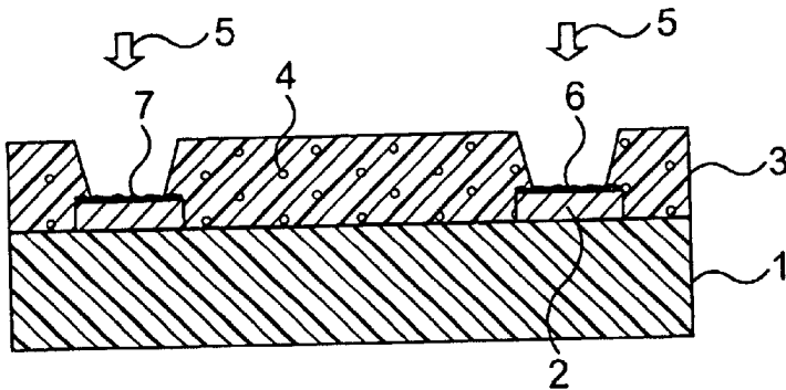
FIG. 4(c) PRIOR ART
