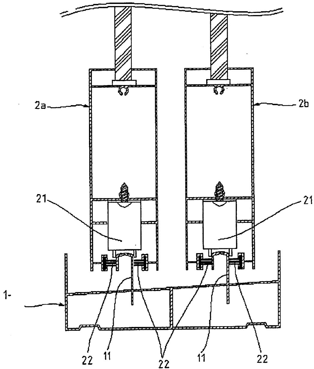
FIG. 2 (Prior Art)
