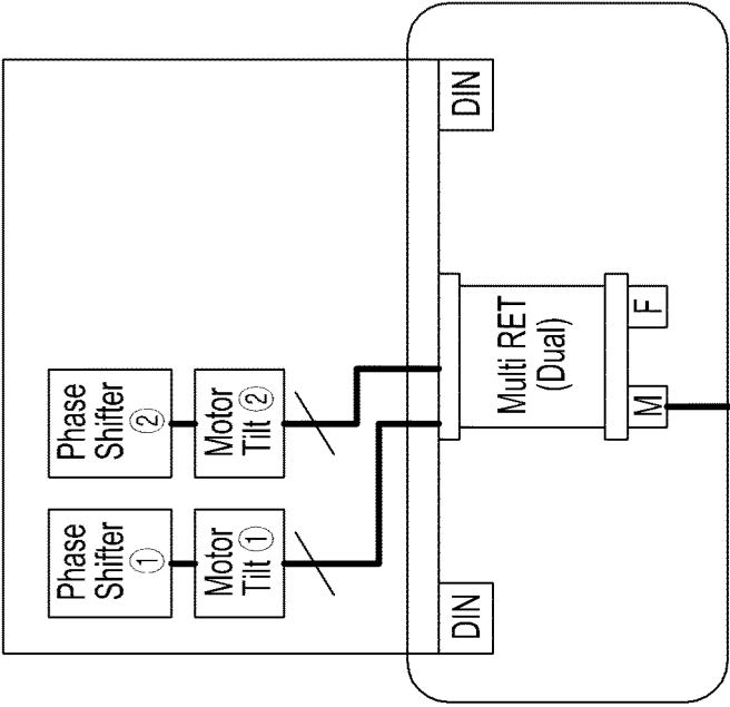
Dual Band Antenna & Multi RET (Dual)
