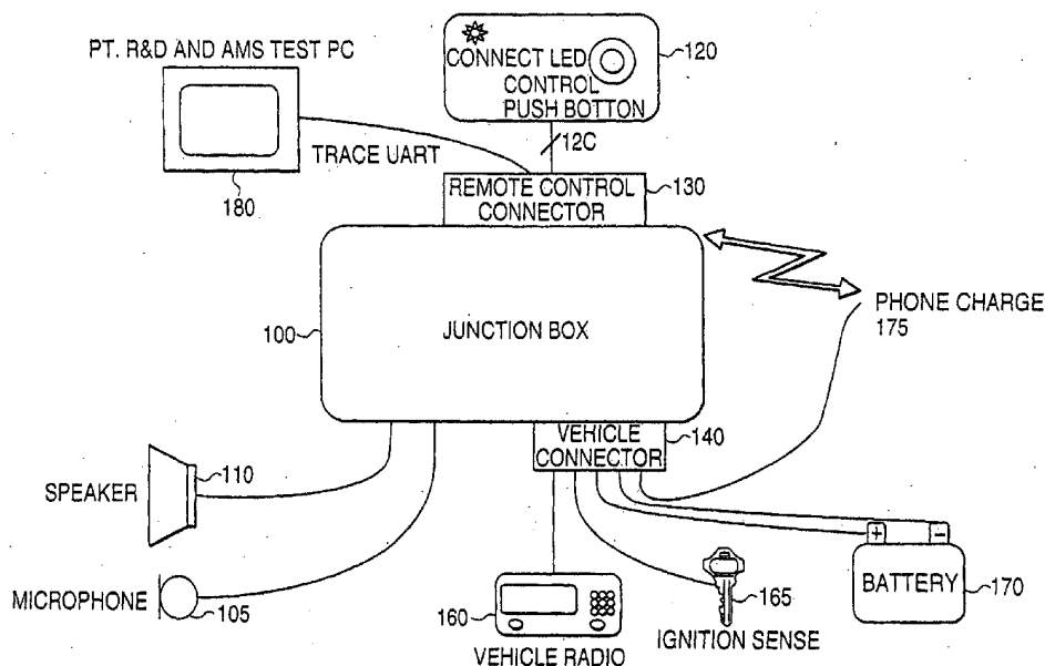
FIG. 1 REMOTE CONTROL
