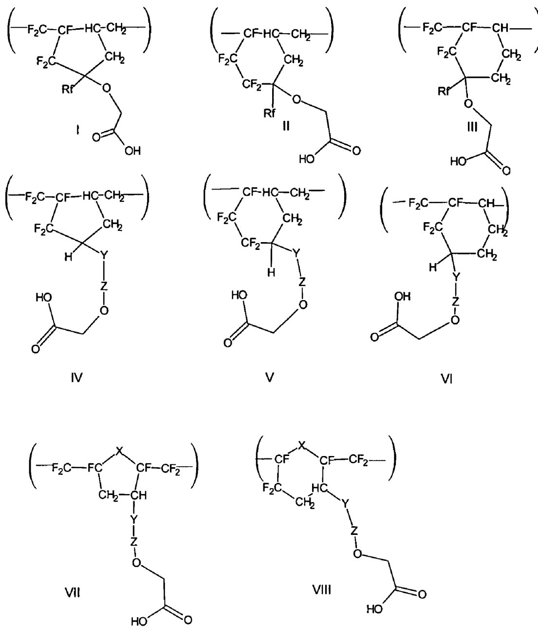
Figure 12: Partially fluorinated monocyclic polymers
