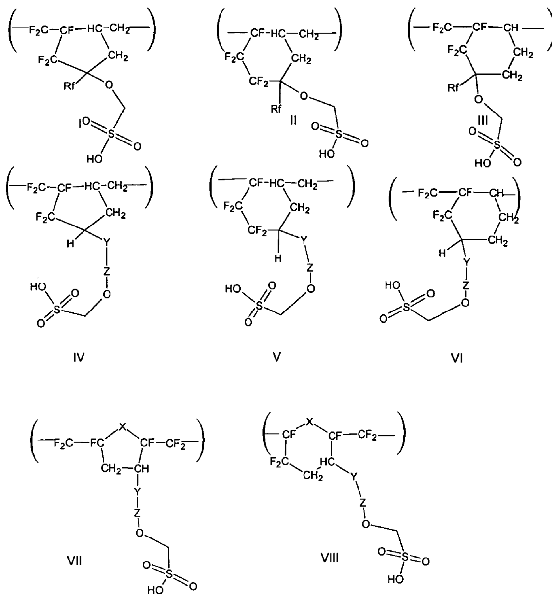
Figure 13: Partially fluorinated monocyclic polymers
