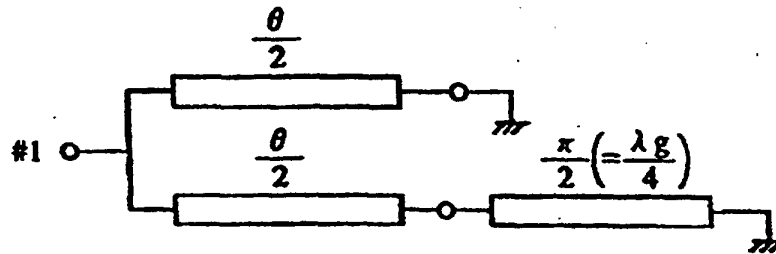
FIG. 24C EQUIVALENT CIRCUIT OF CIRCUIT SHOWN IN FIG. 24A
