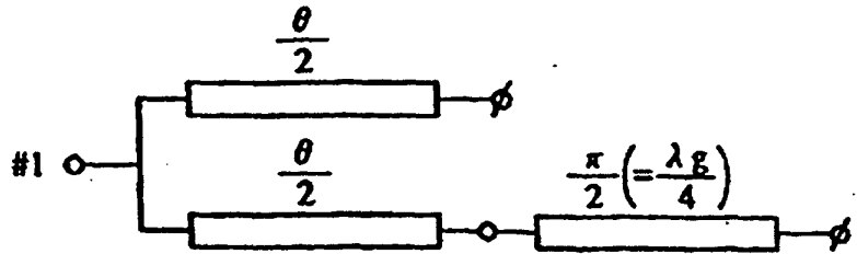
FIG. 24A WHEN PLANE B-B' IS OPEN
