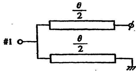
FIG. 24C EQUIVALENT CIRCUIT OF CIRCUIT SHOWN IN FIG. 24A
