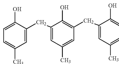
[Chemical Formula 10]
