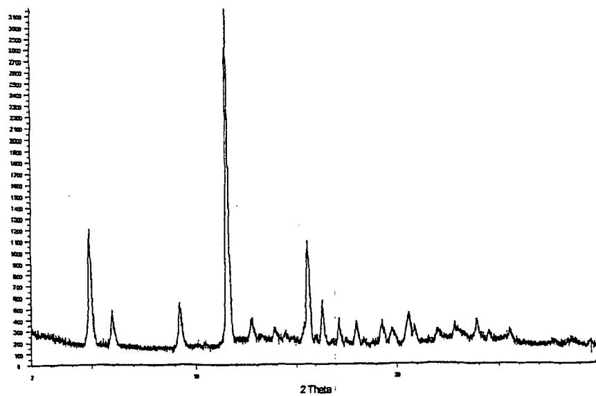
Figure 1.4 Polymorph IV
