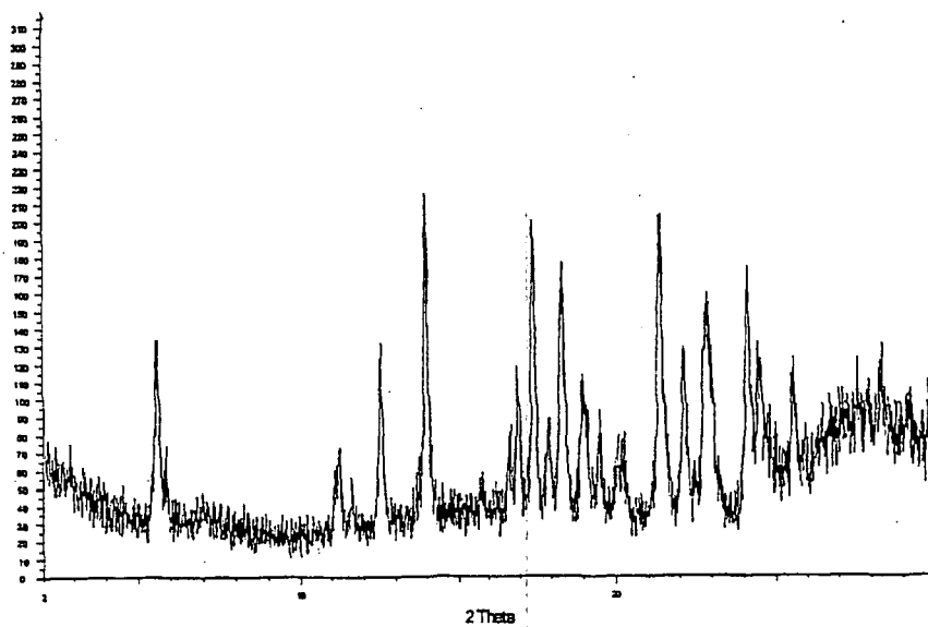
Figure 1.4 Polymorph IV
