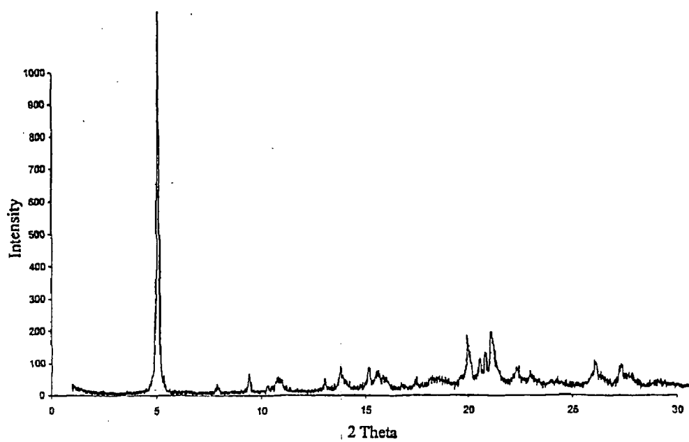
Figure 1.2 Polymorph II
