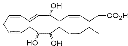
7,16,17-Trihydroxy DTAn-6
