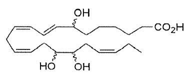
7,16,17-Trihydroxy DTAn-3
