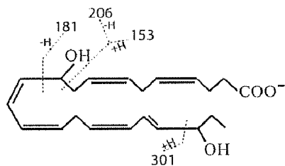
10,20- dihydroxy DHA
