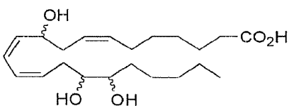
10,16,17-Trihydroxy DTRAn-6
