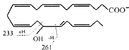
16-hydroxy DHA
