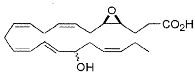
4,5-Epoxy-17-OH DPA
