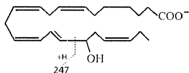
17-hydroxy DPAn-3
