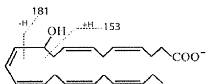
10-hydroxy DHA
