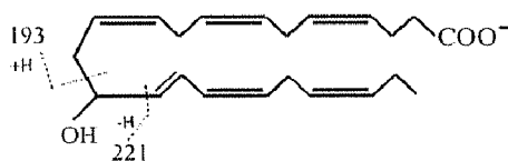
13-hydroxy DHA
