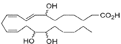
7,16,17-Trihydroxy DTRAn-6
