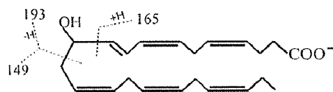
11-hydroxy DHA
