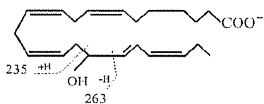
16-hydroxy DPAn-3
