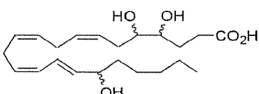
4,5,17-Trihydroxy DTAn-6
