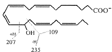
14-hydroxy DPAn-3
