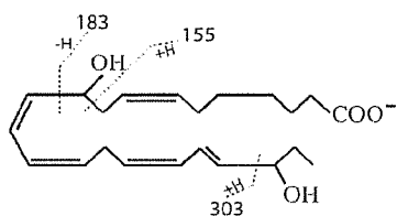
10,20 dihydroxy DPAn-3
