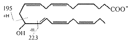
13-hydroxy DPAn-3
