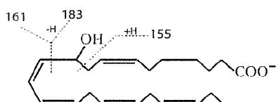
10-hydroxy DPAn-3
