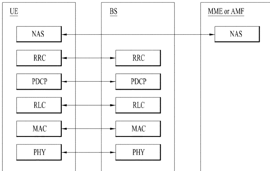
(b) Control Plane Protocol Stack
