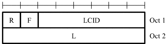
(a) R/F/LCID/L MAC subheader with 8-bit L field
