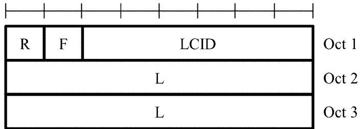
(b) R/F/LCID/L MAC subheader with 16-bit L field
