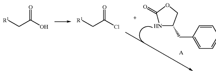
Scheme I. Preparation of Mercaptoketones and Alcohols
