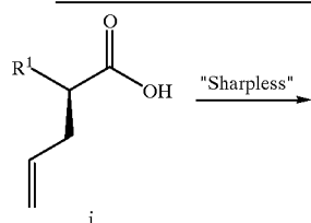
Scheme III. Alternative Preparation of Lactones iii a and iii b
