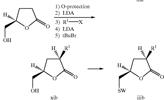
Scheme III. Alternative Preparation of Lactones iii a and iii b
