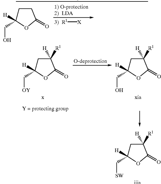
Scheme II. Alternative Preparation of Lactones iii a and iii b
