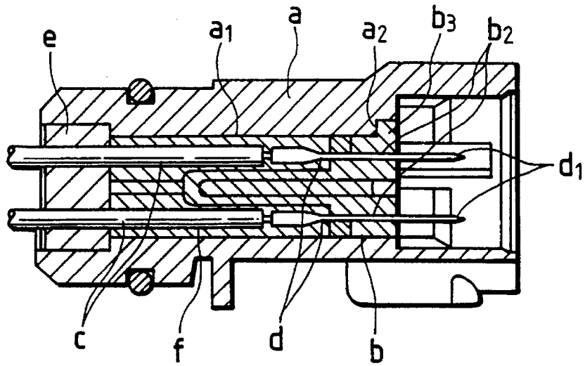
FIG. 5 PRIOR ART
