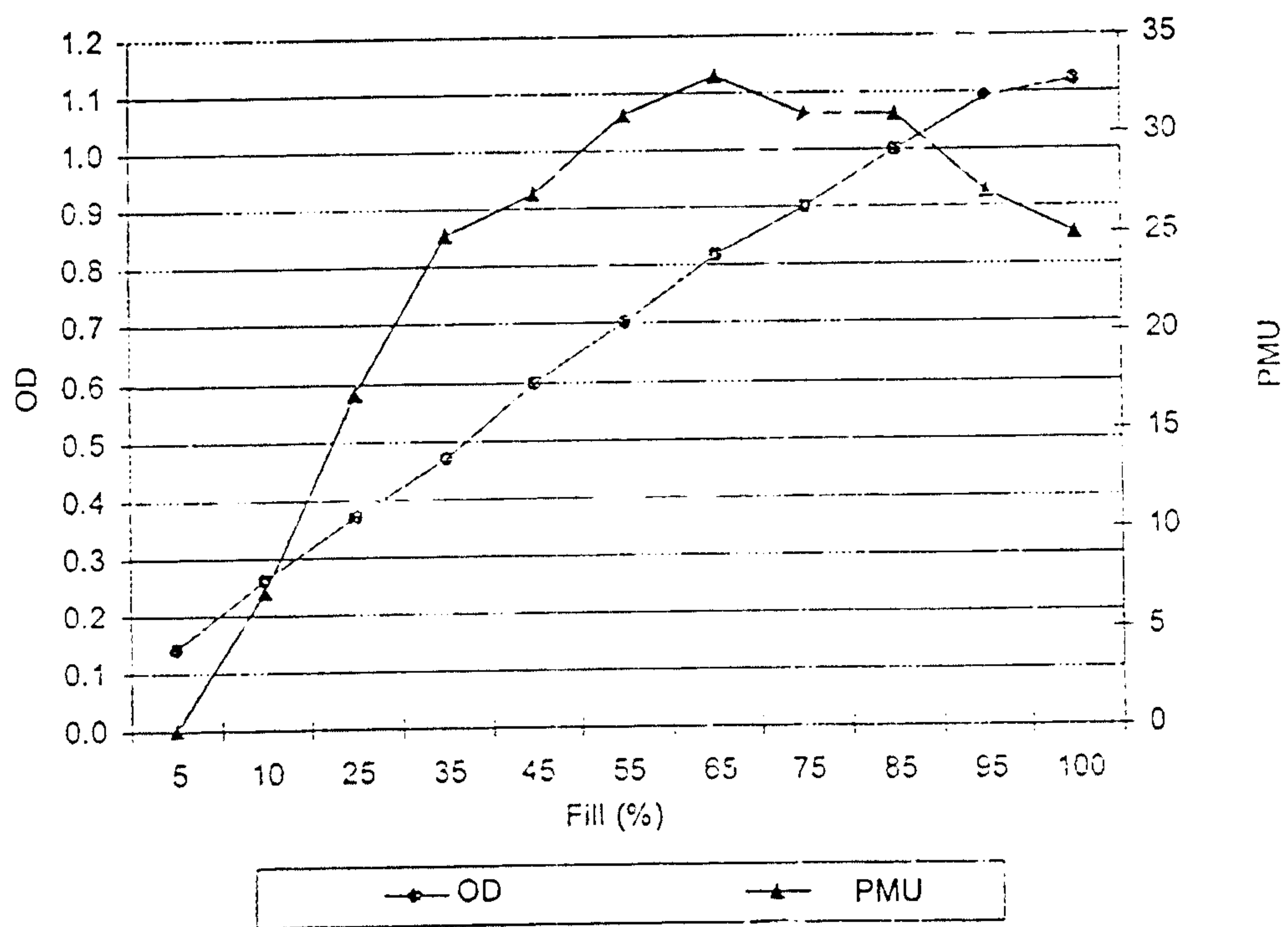
PMU and Optical Density Vs Fill (%) for Ink with AJ Black and CD380 (Printed by Epson C82 Printer, Best Photo)
